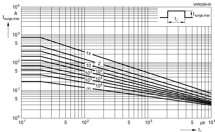
CT1812K14G ... K30G
