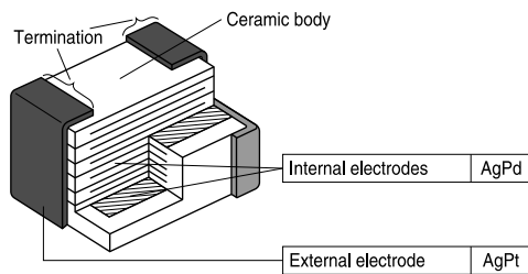
Multilayer varistor: Structure of silver-platinum termination
