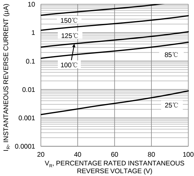
Figure 3. Typical Reverse Characteristics B120Q/BQ - B140Q/BQ
