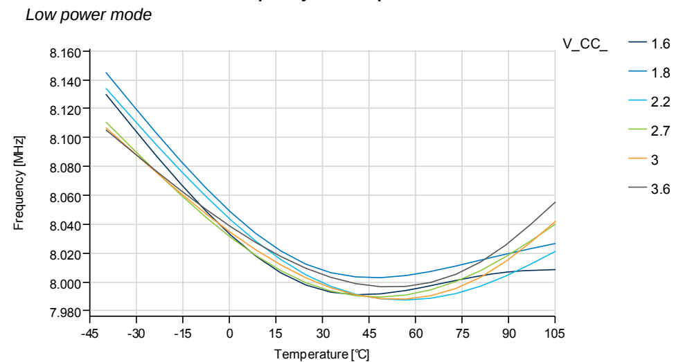
Figure 37-75. 8MHz Internal Oscillator Frequency vs. Temperature
