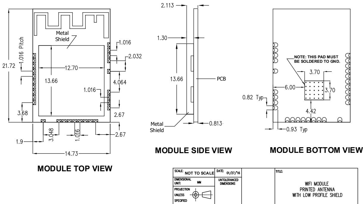
Figure 11-1. Module Drawings – ATWILC1000-MR110PB - Top, Bottom and Side Views
