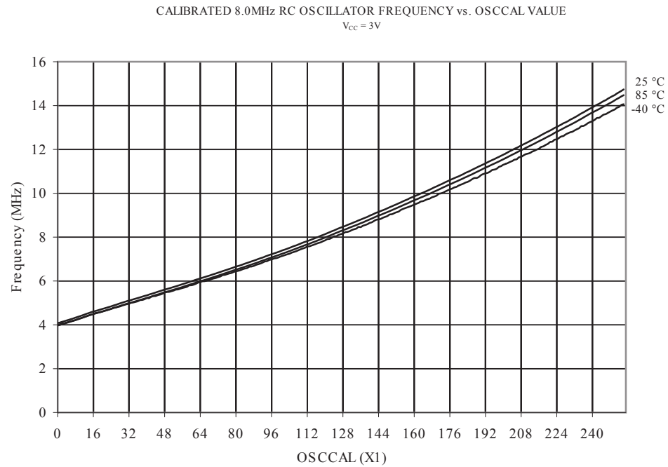
Figure 19-41 Calibrated Oscillator Frequency vs. OSCAL Value
