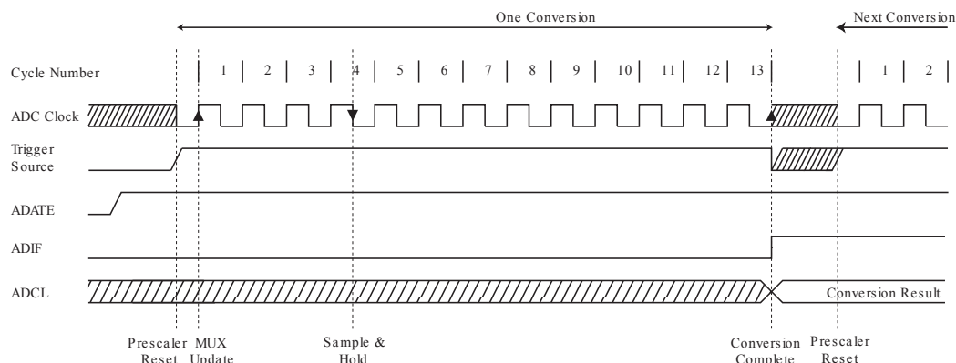
Figure 15-6 ADC Timing Diagram, Auto Triggered Conversion
