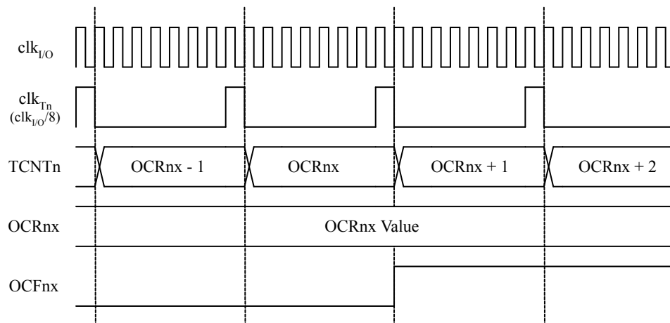
Figure 13-13 Timer/Counter Timing Diagram, Setting of OCF0x, with Prescaler ( f_{\text{clk\_I/O}}/8 )
