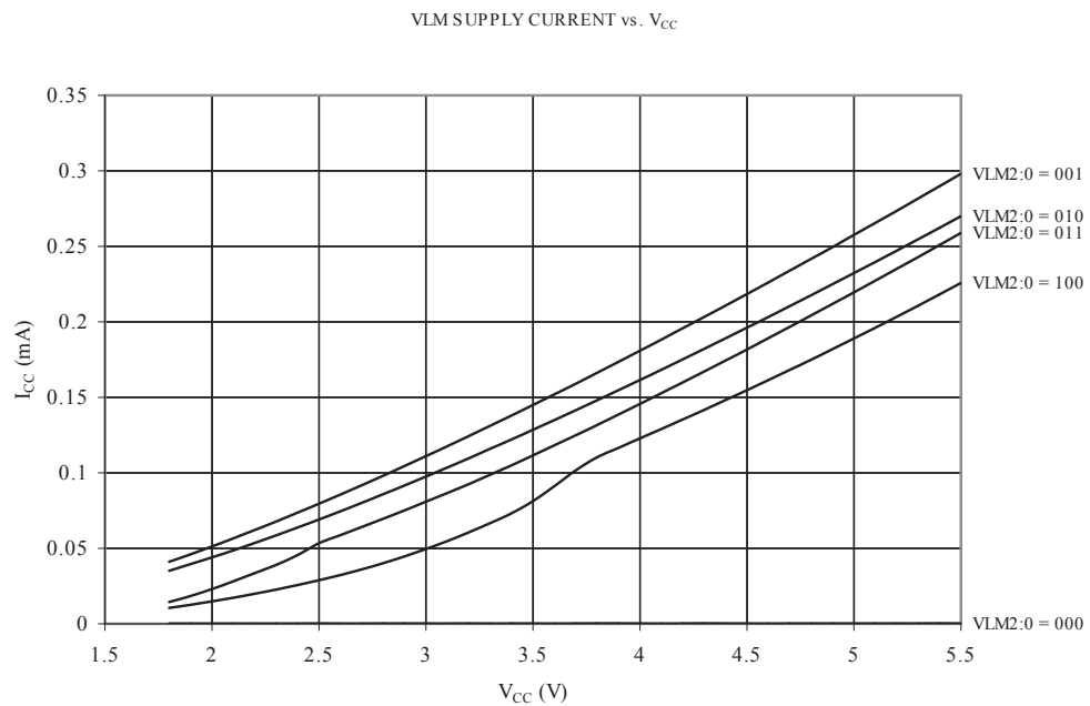
Figure 19-48 V_{CC} Level Monitor Current vs. V_{CC}
