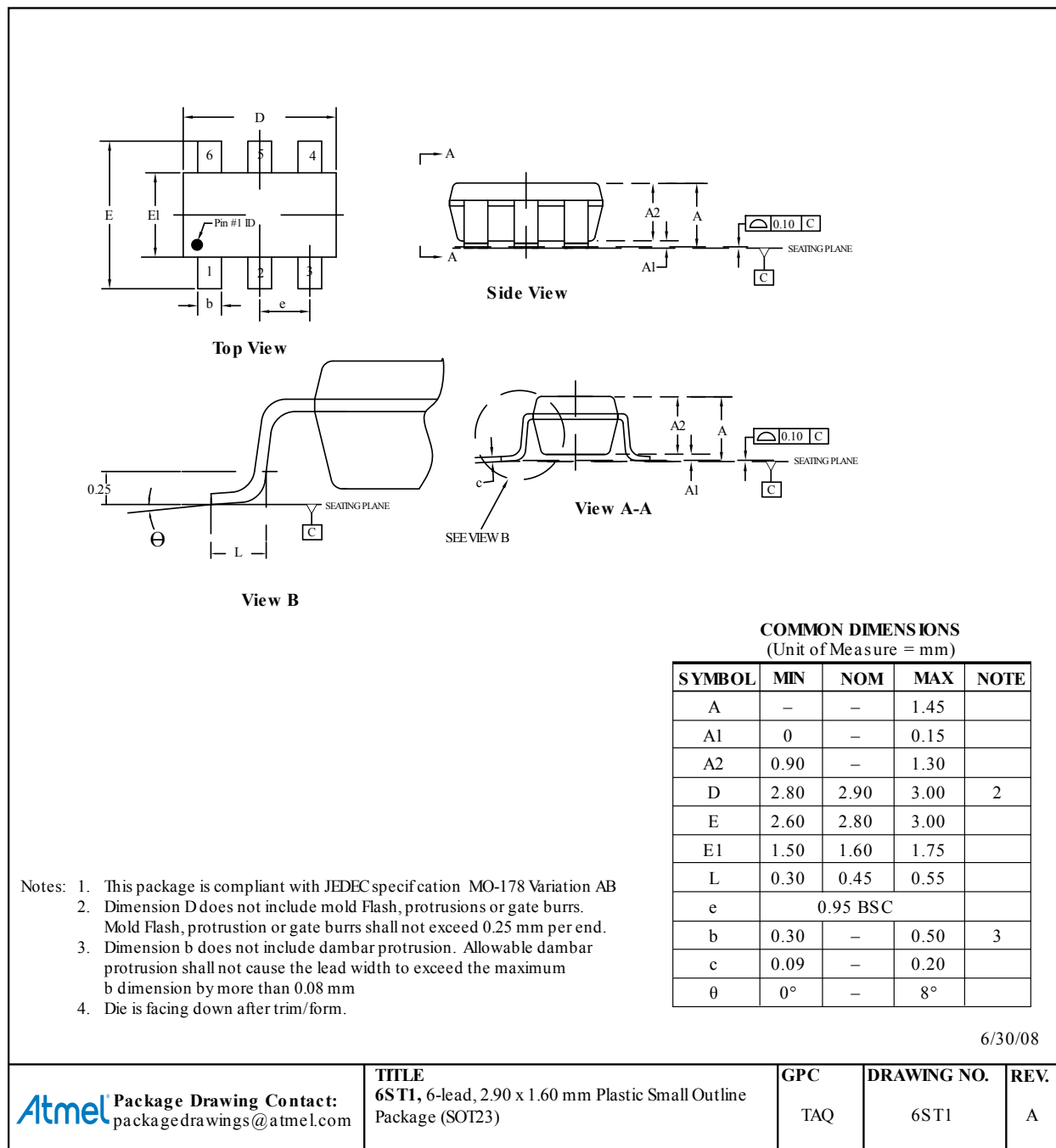
Figure 21-1 6ST1
