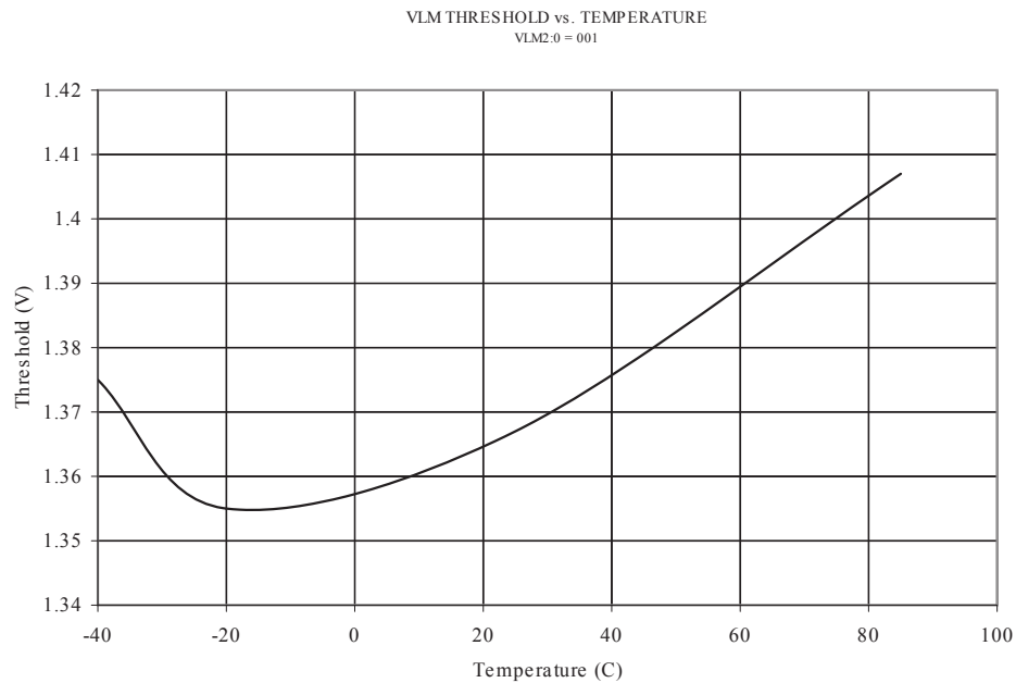
Figure 19-42 VLM1L Threshold of V CC Level Monitor
