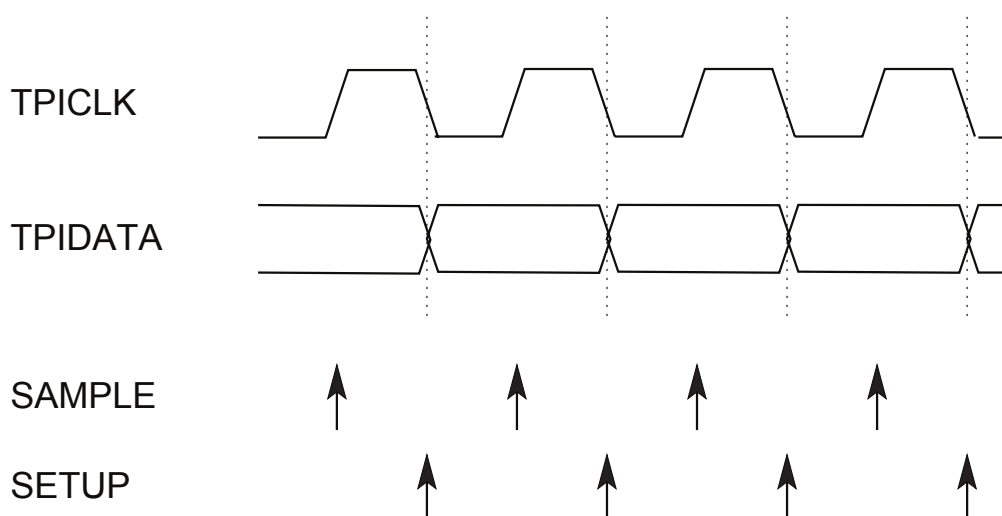
Figure 16-6 Data changing and Data sampling.
