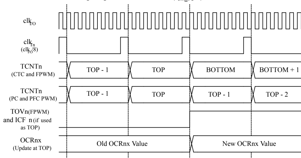
Figure 13-15 Timer/Counter Timing Diagram, with Prescaler ( f_{clk\_I/O}/8 )
