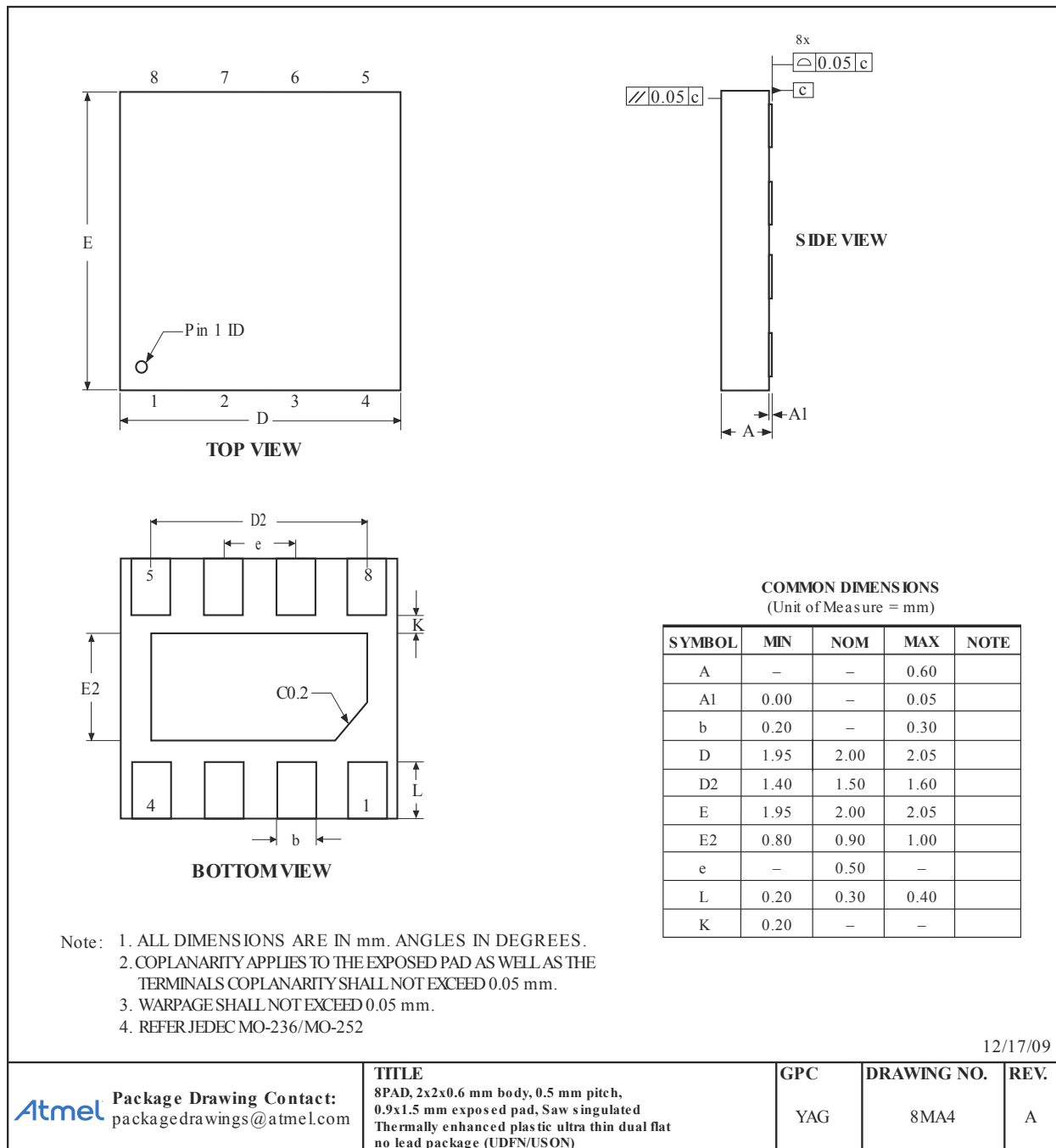
Figure 21-2 8MA4
