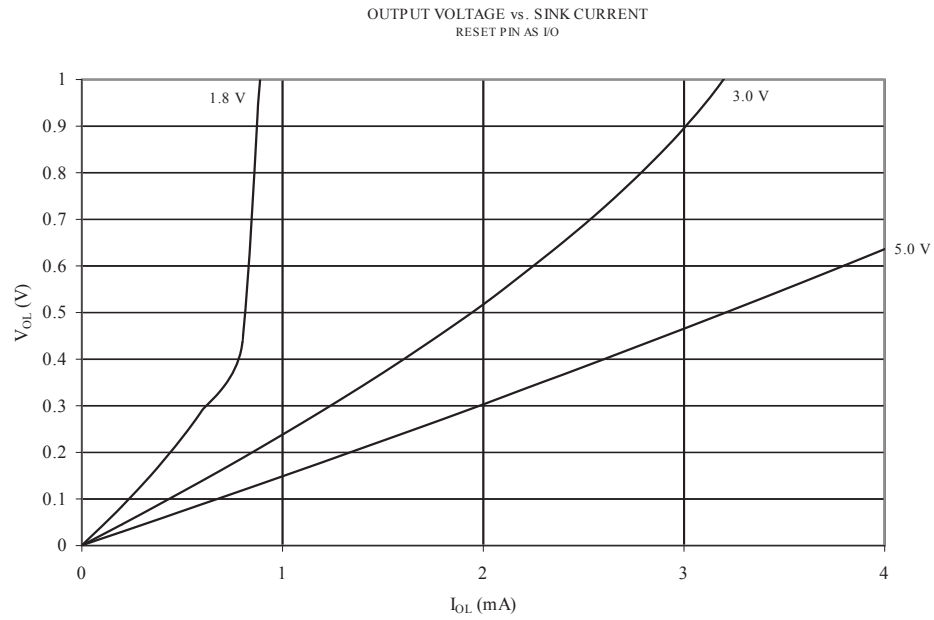
Figure 19-25 Reset Pin as I/O, Output Voltage vs. Sink Current
