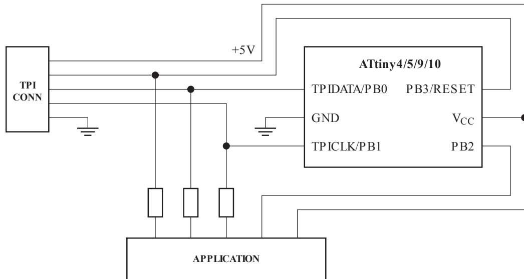
Figure 16-2 Using an External Programmer for In-System Programming via TPI
