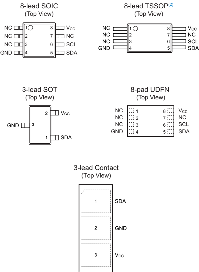
Figure 1. Pinouts (1)
