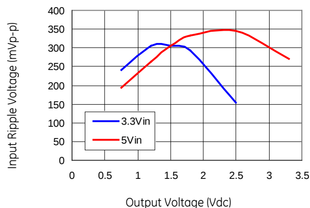
Figure 26. Input ripple voltage for various output with 1x150 μF polymer and 1x47 μF ceramic capacitors at the input (full load).
