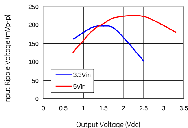
Figure 27. Input ripple voltage for various output with 2x150 μF polymer and 2x47 μF ceramic capacitors at the input (full load).
