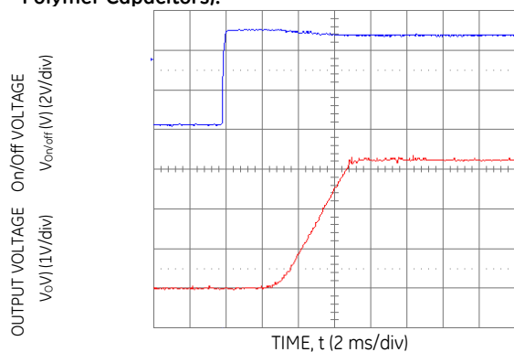
Figure 14. Typical Start-Up Using Remote On/Off ( V_{in} = 5.0 Vdc, V_o = 3.3 Vdc, I_o = 16.0 A).
