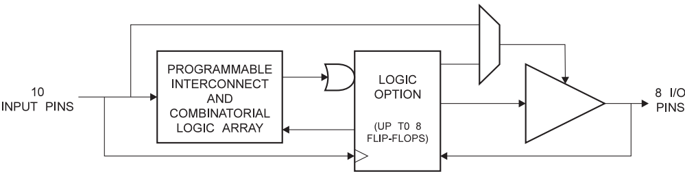
Figure 1-1. Block Diagram
