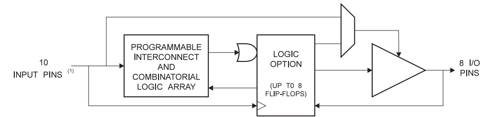
Figure 0-1. Block diagram
