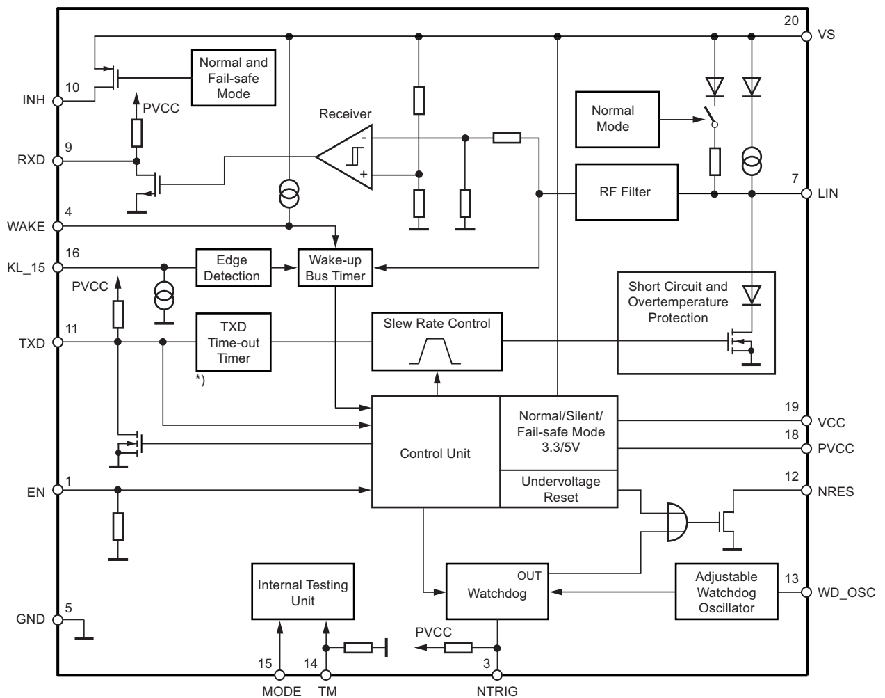
Figure 1-1. Block Diagram
