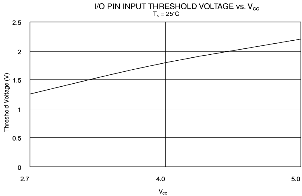
Figure 85. I/O Pin Input Threshold Voltage vs. V_{CC}
