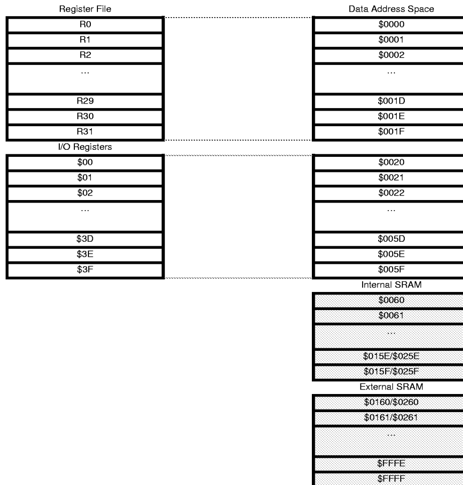
Figure 8. SRAM Organization
