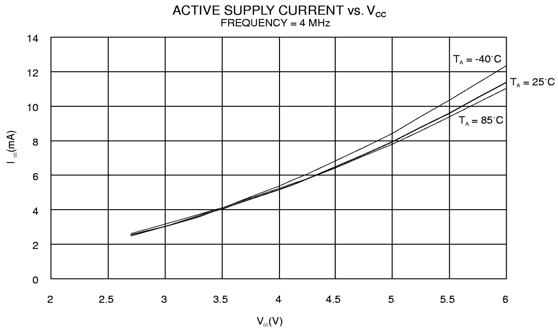
Figure 70. Active Supply Current vs. V_{CC}
