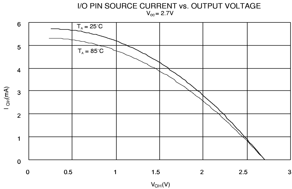
Figure 84. I/O Pin Source Current vs. Output Voltage
