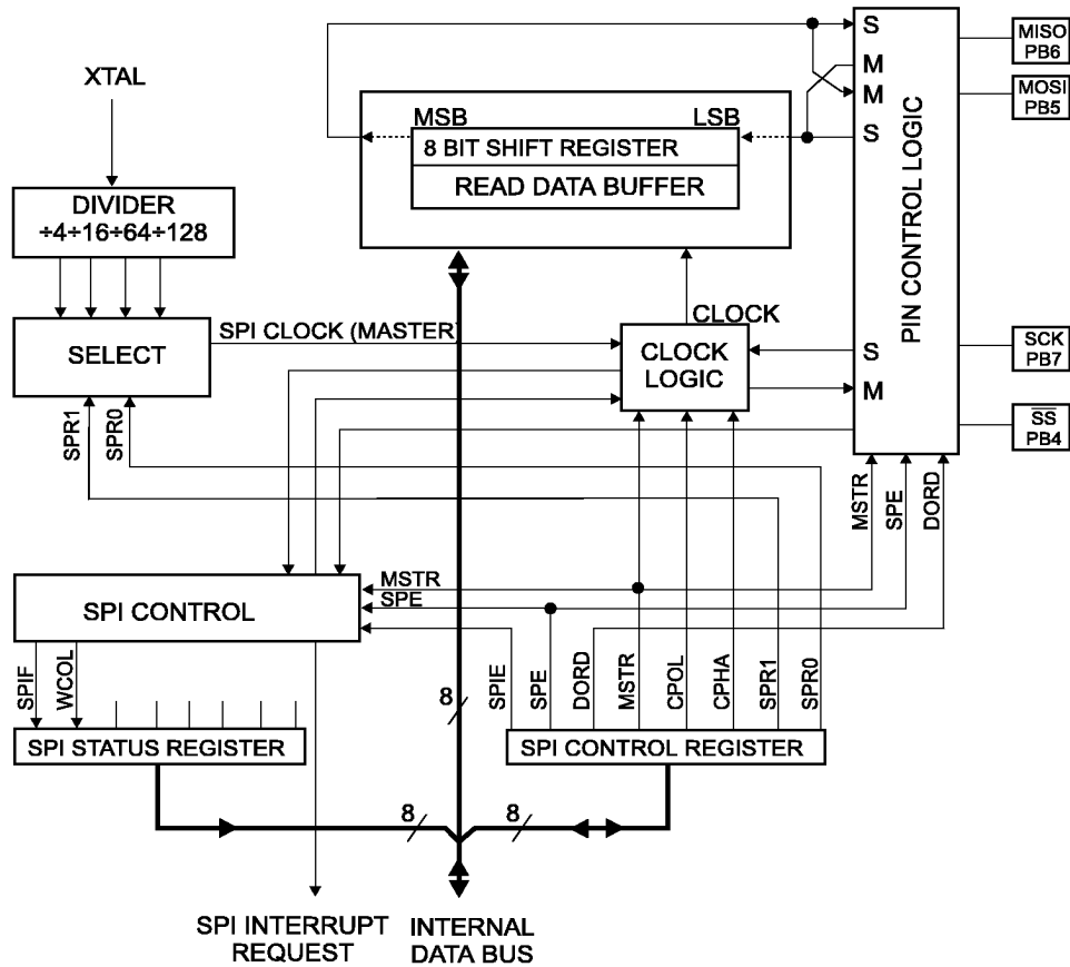
Figure 34. SPI Block Diagram
