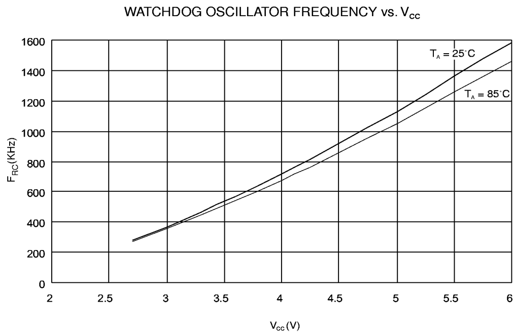
Figure 79. Watchdog Oscillator Frequency vs. V_{CC}
