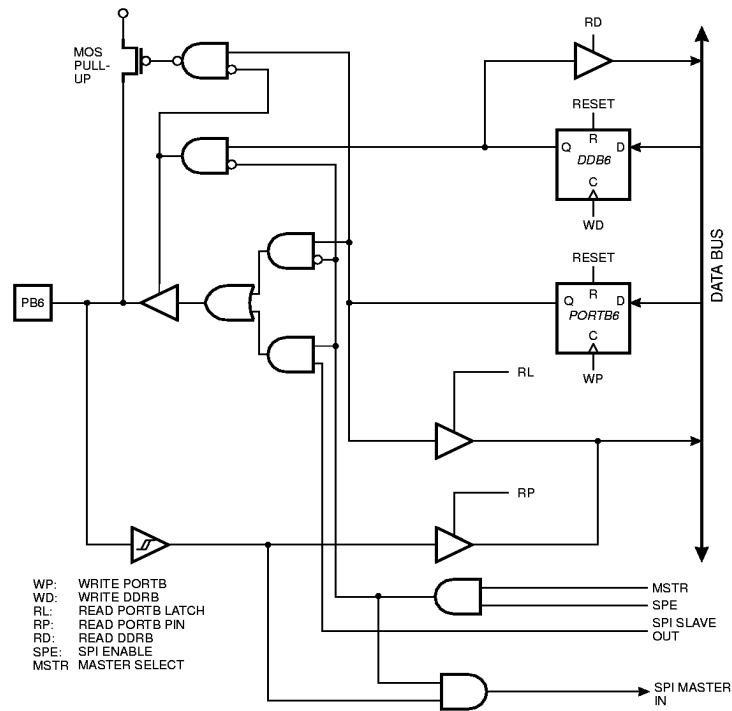
Figure 50. Port B Schematic Diagram (Pin PB6)
