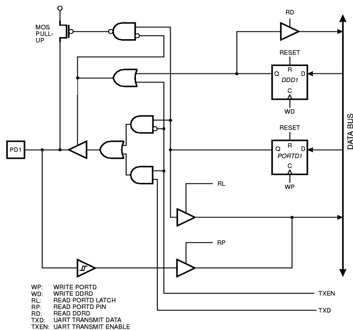
Figure 54. Port D Schematic Diagram (Pin PD1)
