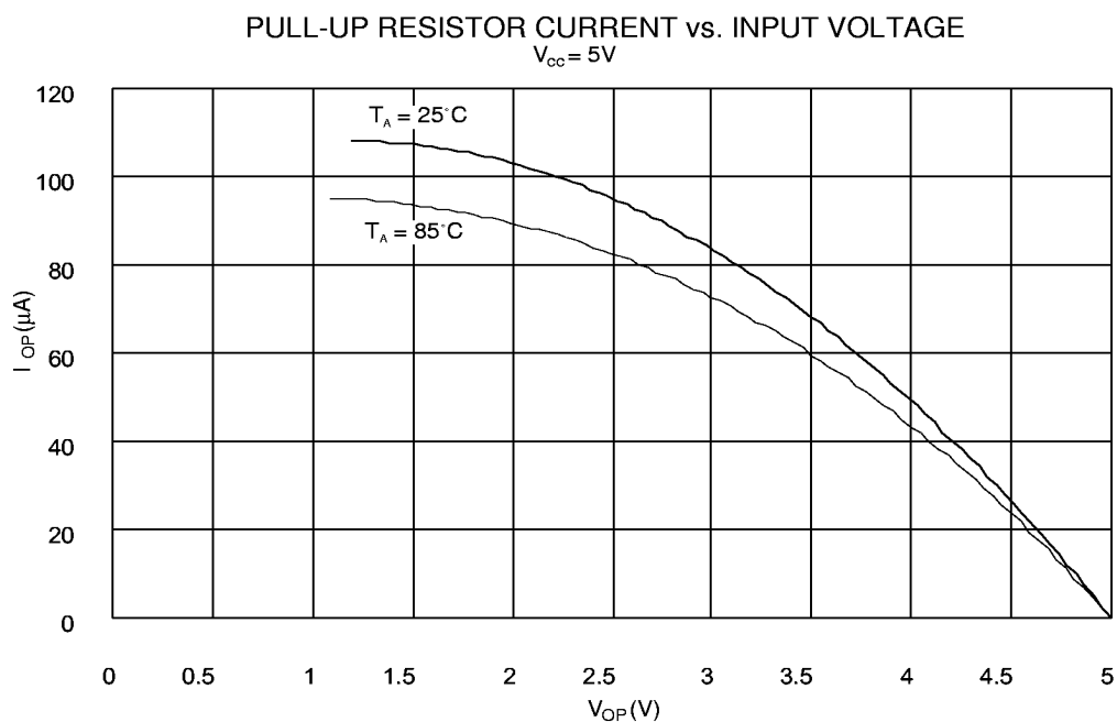
Figure 80. Pull-up Resistor Current vs. Input Voltage
