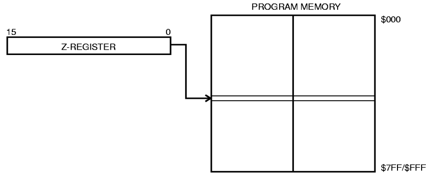
Figure 18. Indirect Program Memory Addressing
