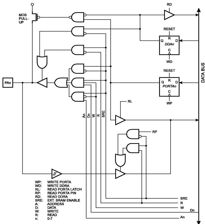
Figure 45. Port A Schematic Diagrams (Pins PA0 - PA7)
