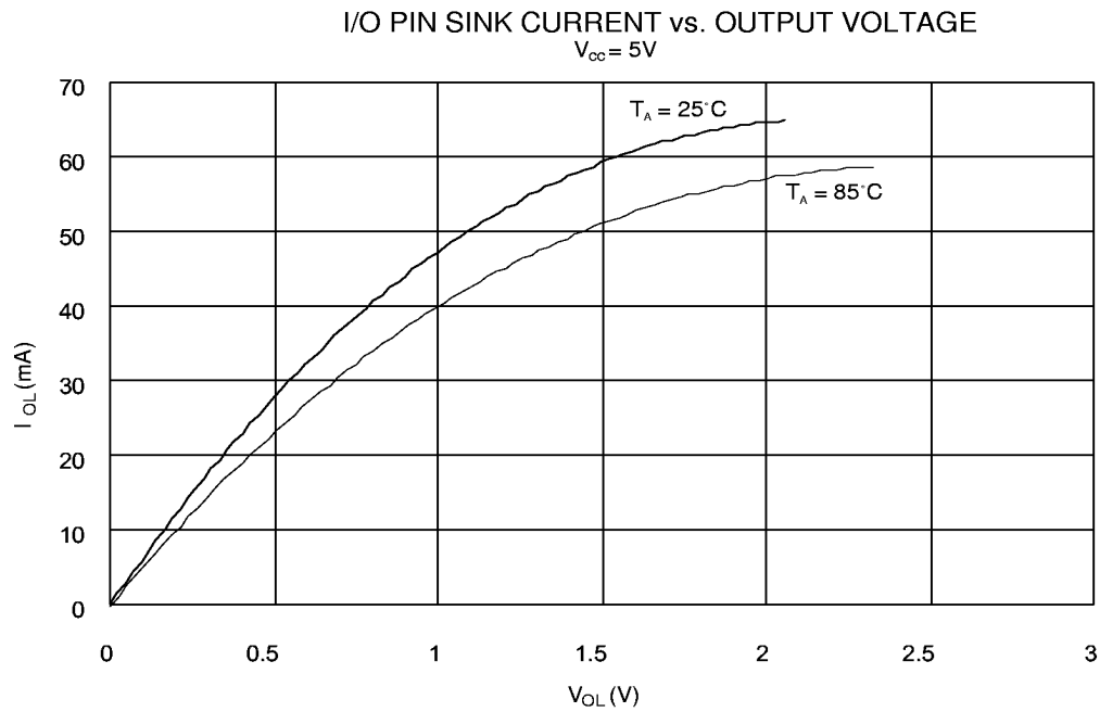
Figure 82. I/O Pin Sink Current vs. Output Voltage
