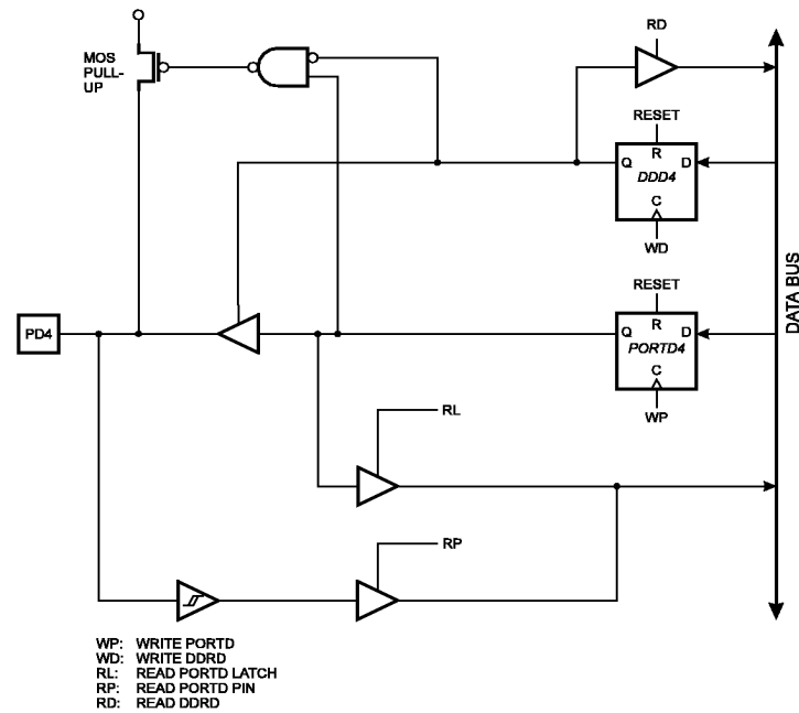
Figure 56. Port D Schematic Diagram (Pin PD4)
