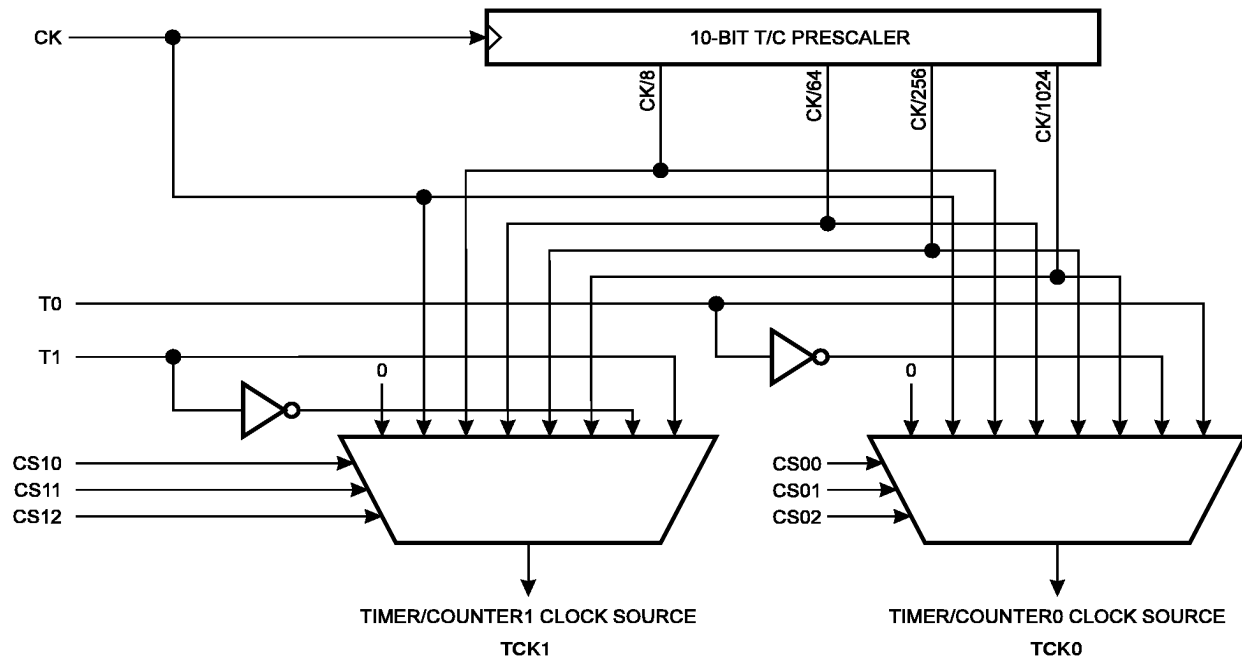
Figure 28. Timer/Counter Prescaler
