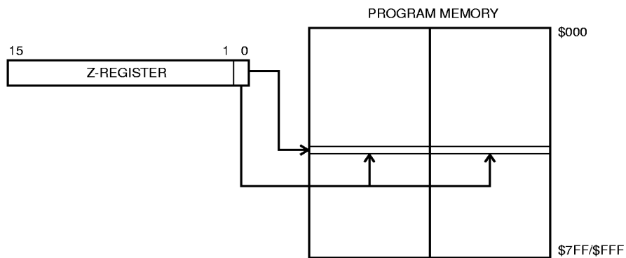
Figure 17. Code Memory Constant Addressing
