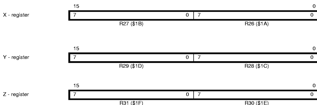
Figure 7. X, Y and Z Registers
