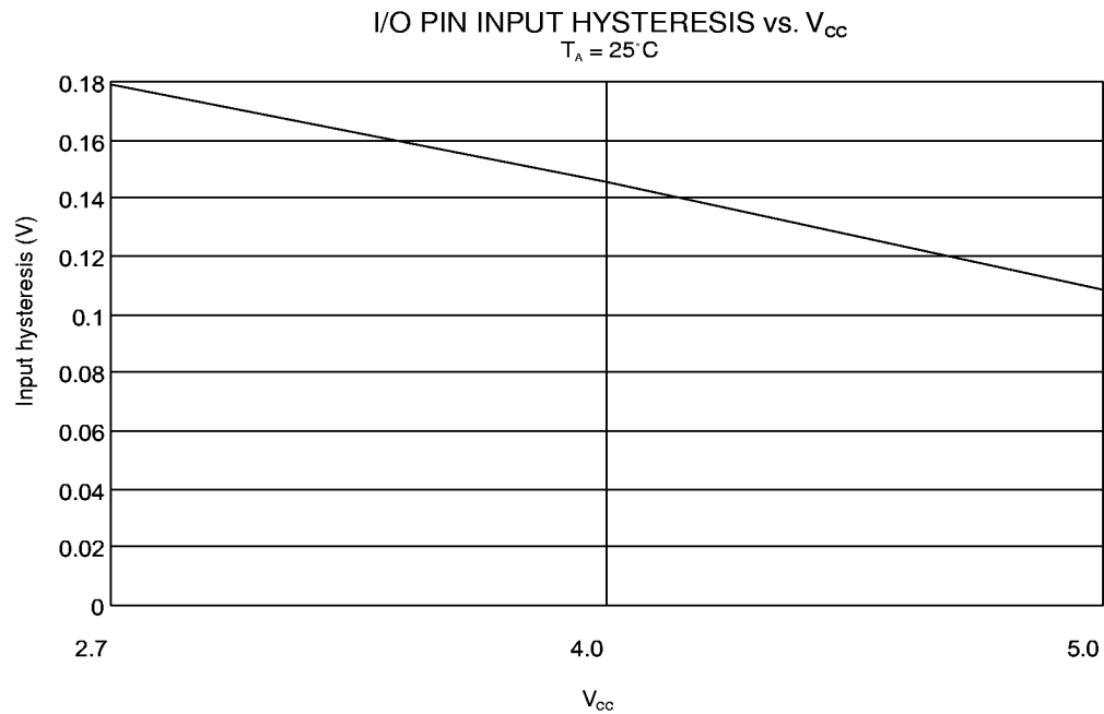
Figure 86. I/O Pin Input Hysteresis vs. V_{CC}
