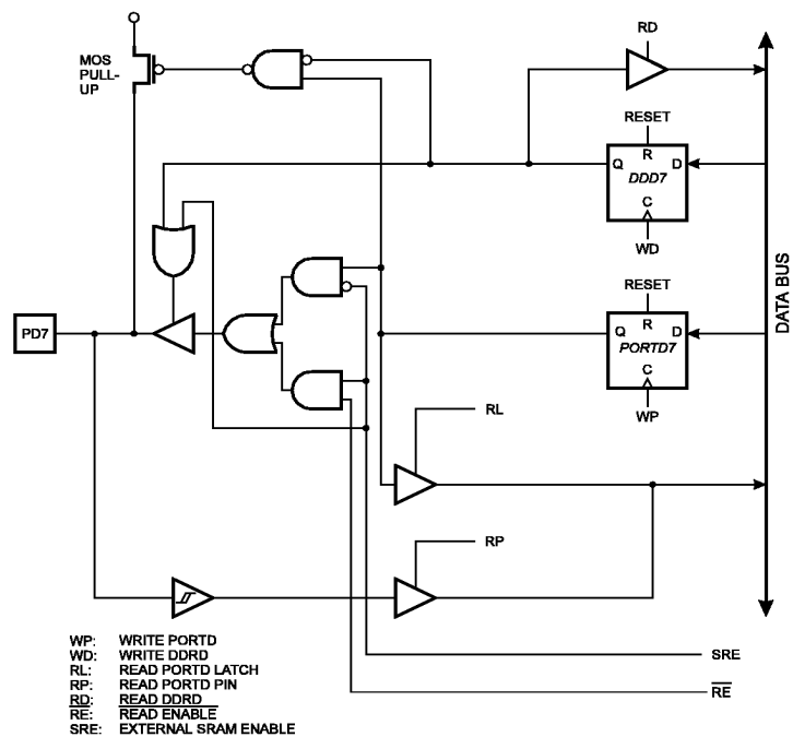
Figure 59. Port D Schematic Diagram (Pin PD7)
