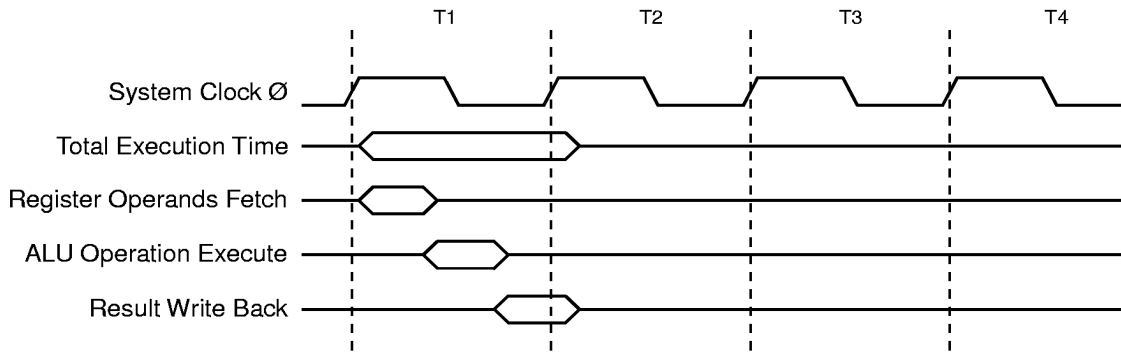
Figure 21. Single Cycle ALU Operation
