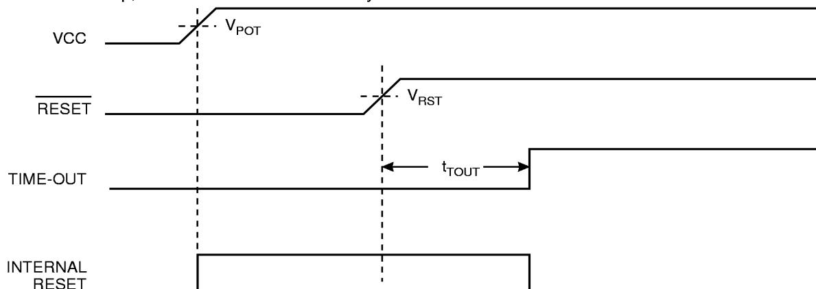
Figure 25. MCU Start-up, \overline{RESET} Controlled Externally
