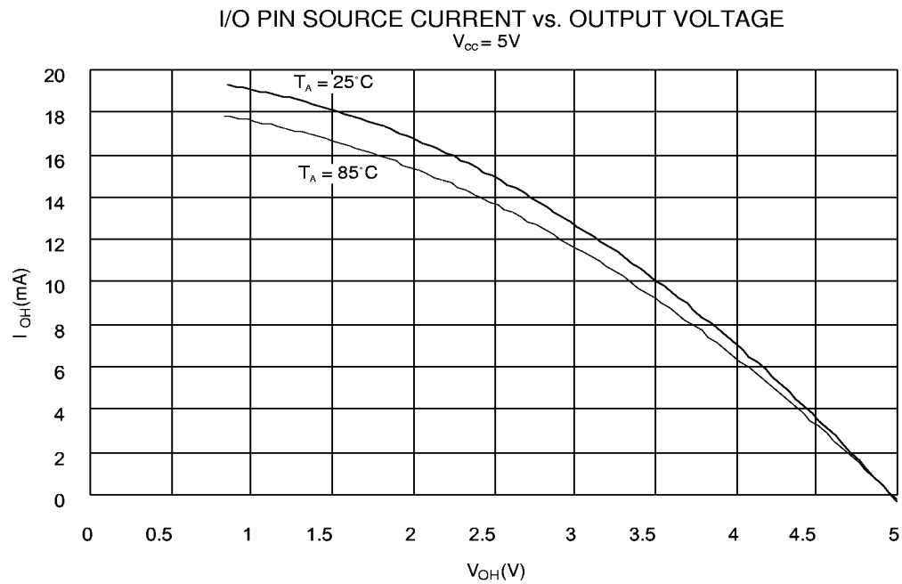
Figure 83. I/O Pin Source Current vs. Output Voltage
