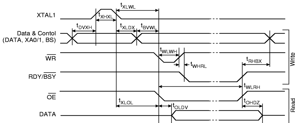
Figure 63. Parallel Programming Timing
