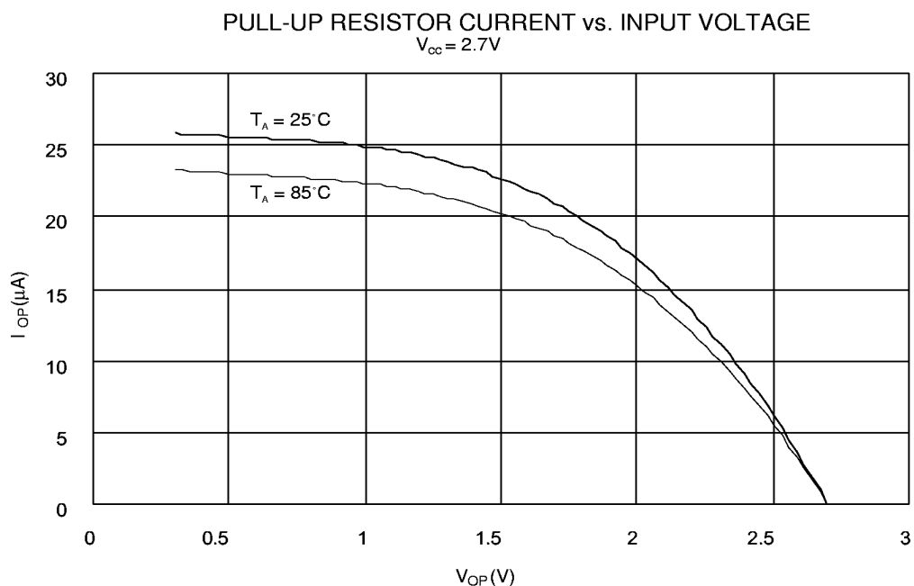
Figure 81. Pull-up Resistor Current vs. Input Voltage
