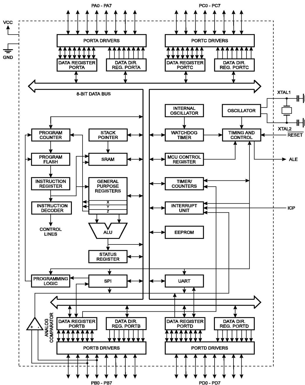
Figure 1. The AT90S4414/8515 Block Diagram
