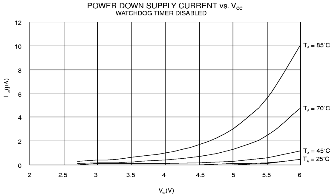
Figure 73. Power Down Supply Current vs. V_{CC}
