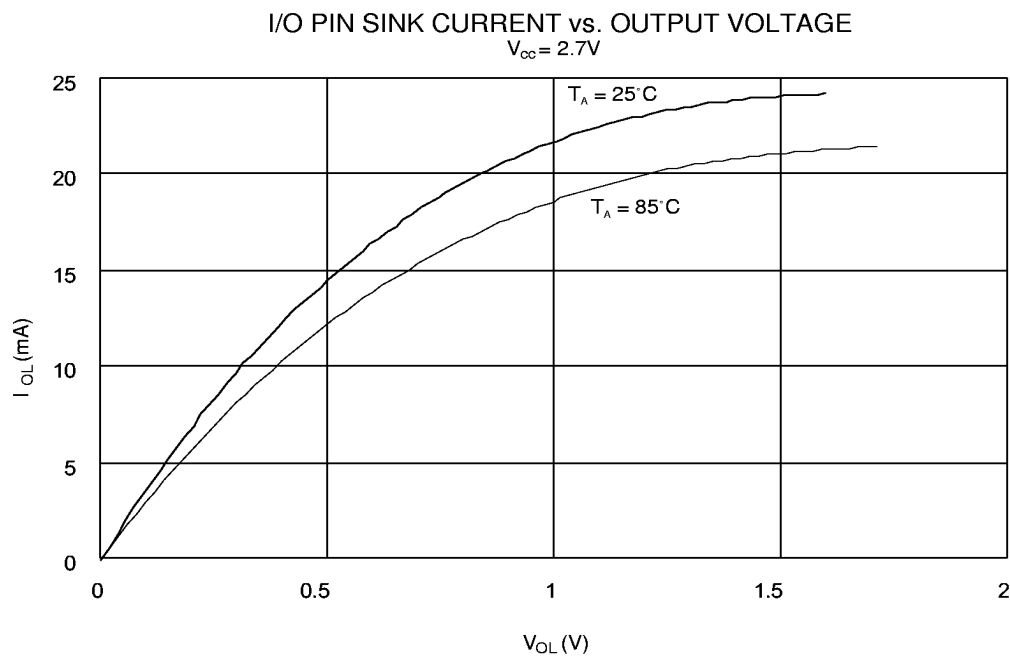
Figure 87. I/O Pin Sink Current vs. Output Voltage
