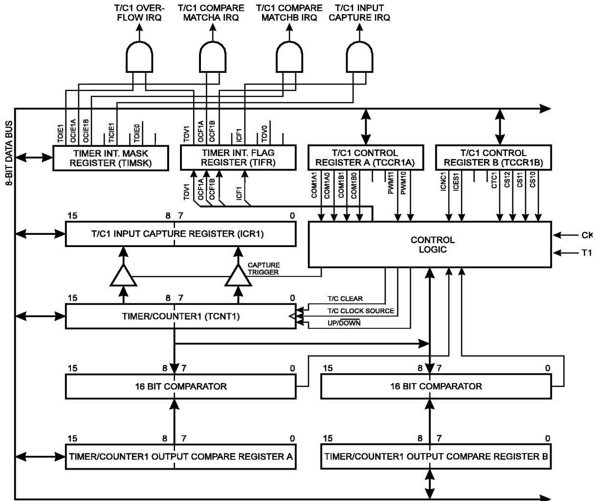
Figure 30. Timer/Counter1 Block Diagram
