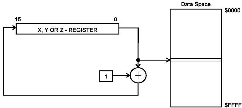
Figure 16. Data Indirect Addressing with Post-increment
