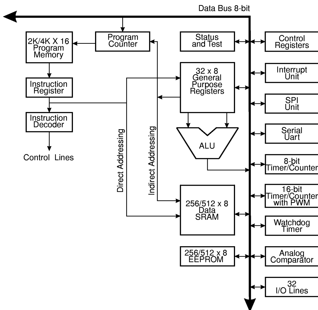
Figure 4. The AT90S4414/8515 AVR RISC Architecture
