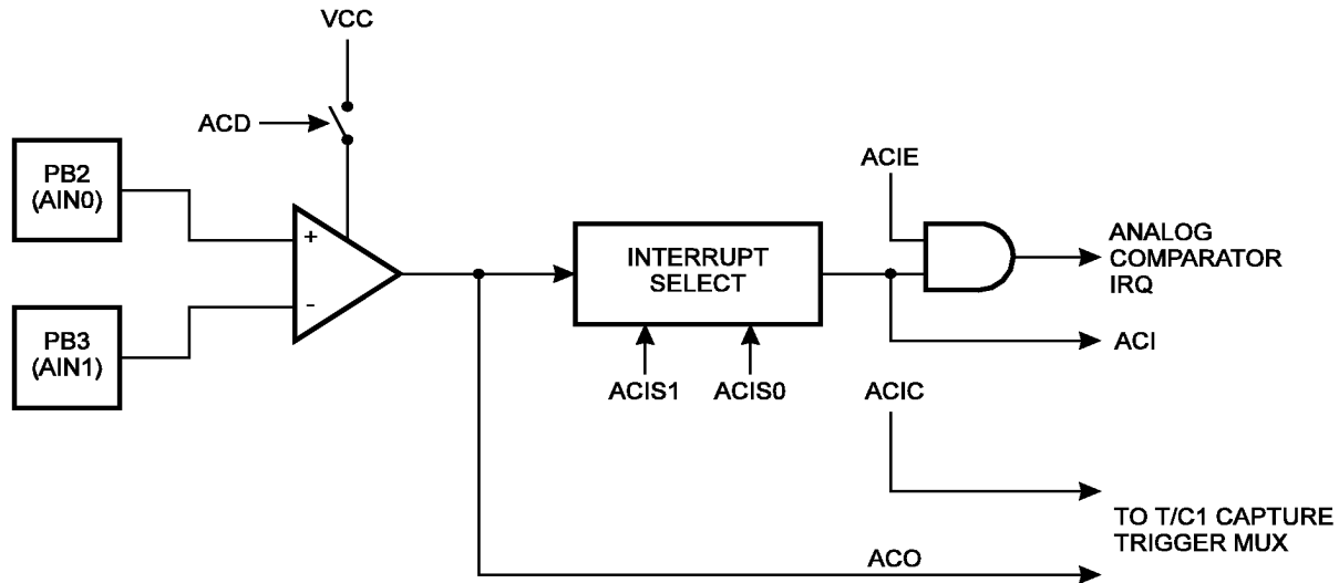
Figure 41. Analog Comparator Block Diagram
