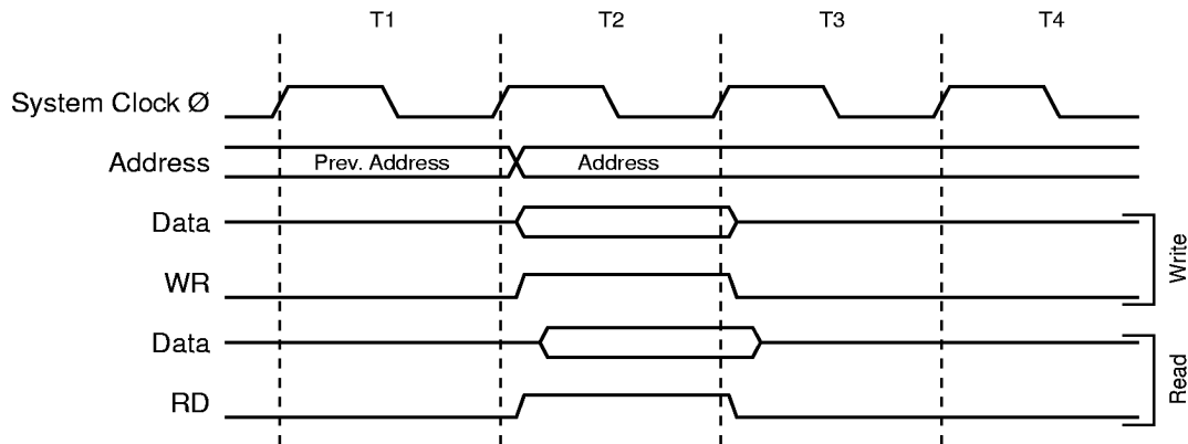
Figure 22. On-chip Data SRAM Access Cycles
