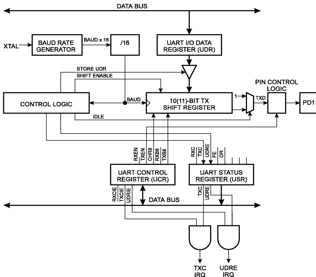
Figure 38. UART Transmitter
