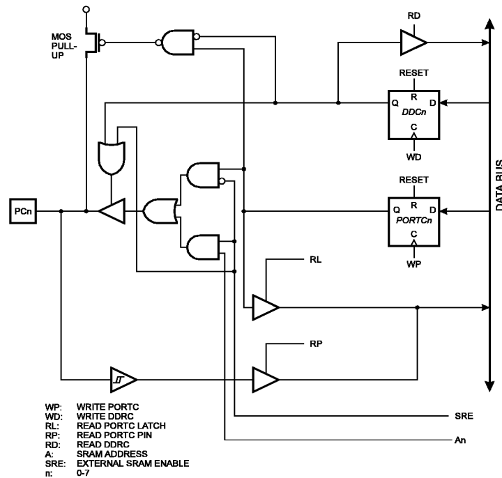
Figure 52. Port C Schematic Diagram (Pins PC0 - PC7)
