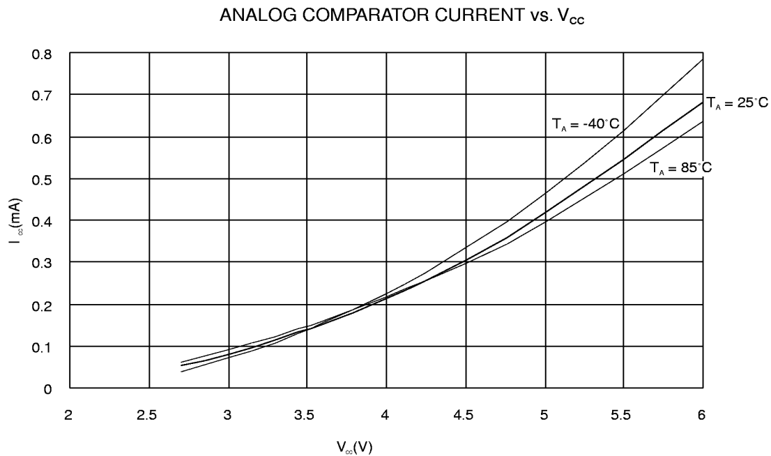
Figure 75. Analog Comparator Current vs. V_{CC}
