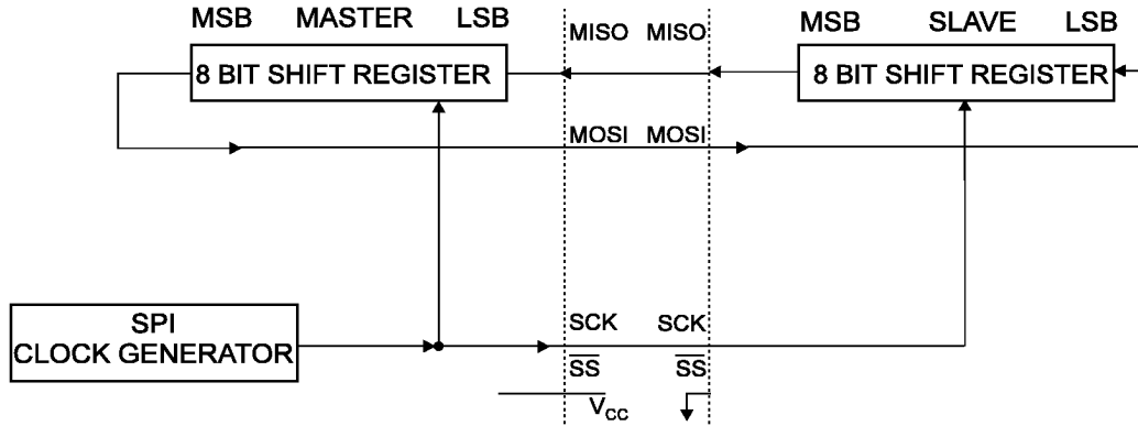
Figure 35. SPI Master-slave Interconnection
