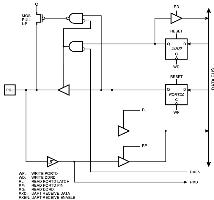
Figure 53. Port D Schematic Diagram (Pin PD0)
