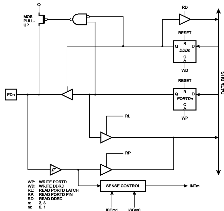
Figure 55. Port D Schematic Diagram (Pins PD2 and PD3)
