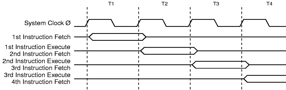
Figure 20. The Parallel Instruction Fetches and Instruction Executions
