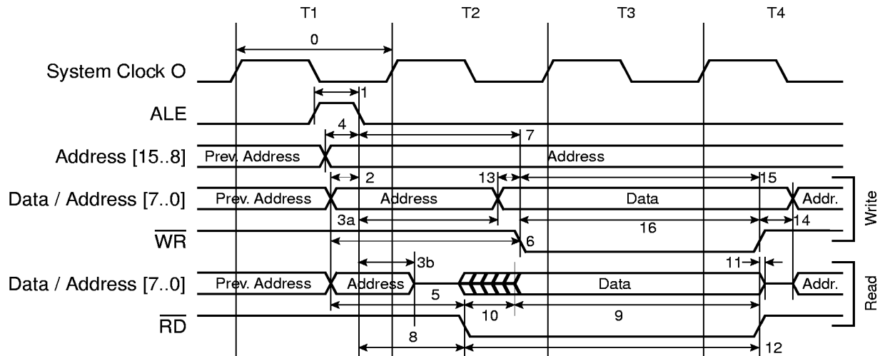
Figure 68. External RAM Timing
