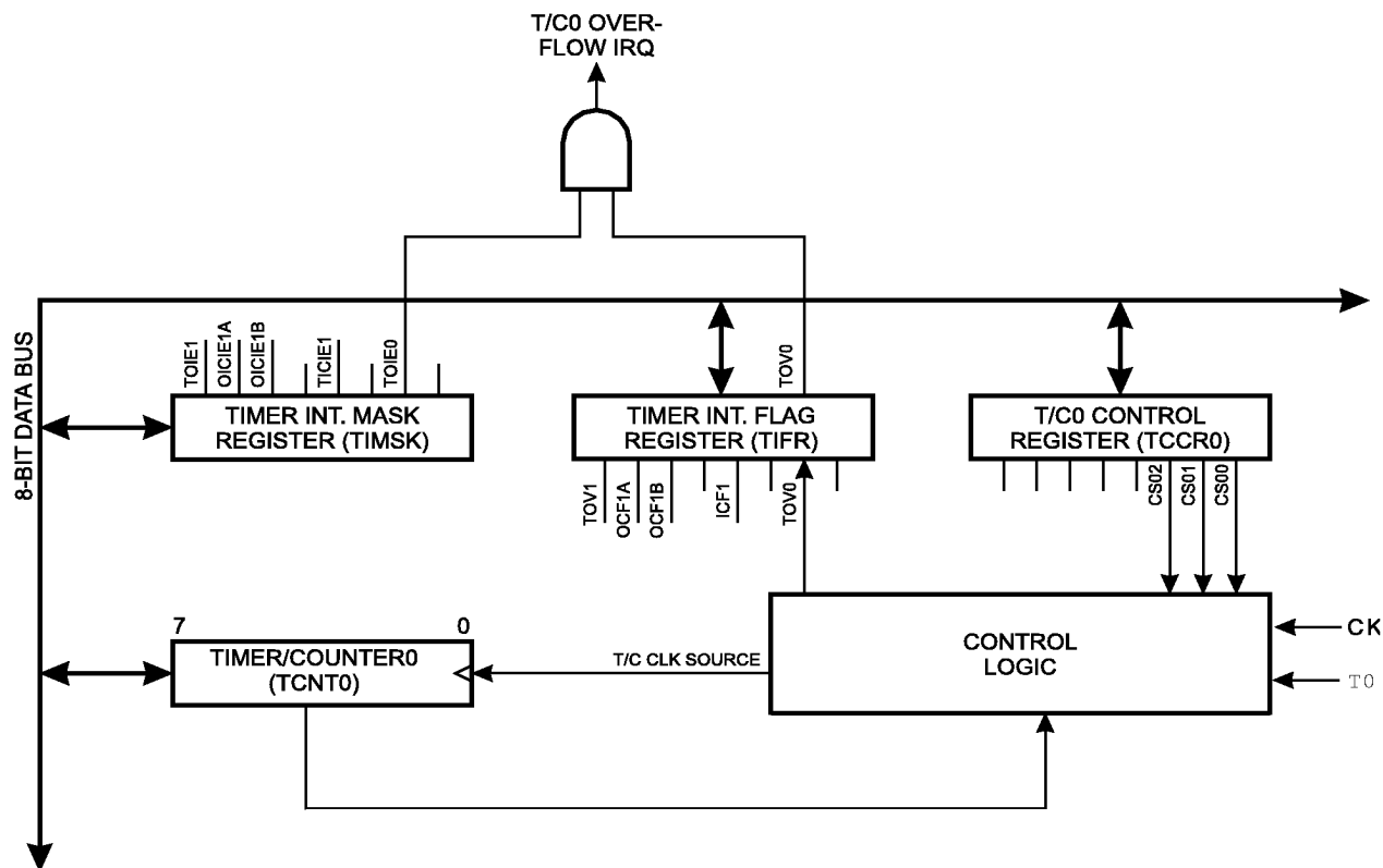
Figure 29. Timer/Counter0 Block Diagram
