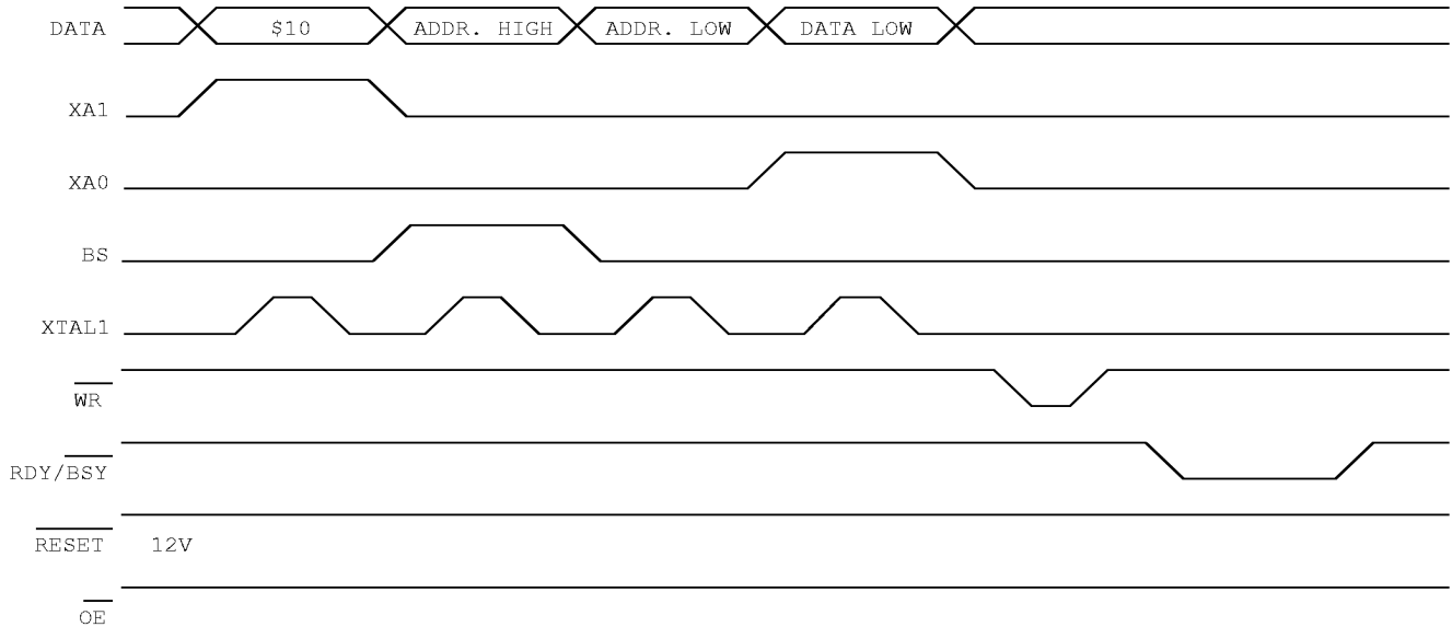
Figure 61. Programming the Flash Waveforms
