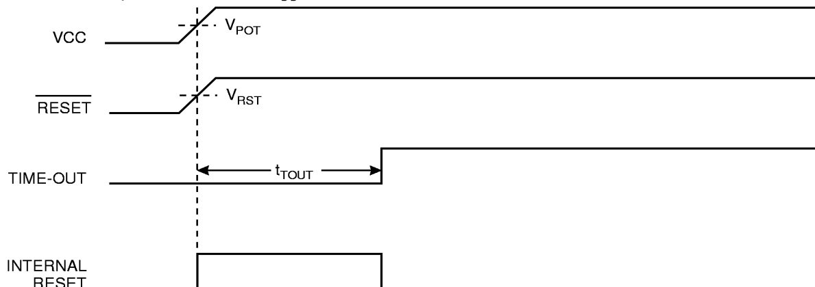
Figure 24. MCU Start-up, \overline{RESET} Tied to V_{CC} .
