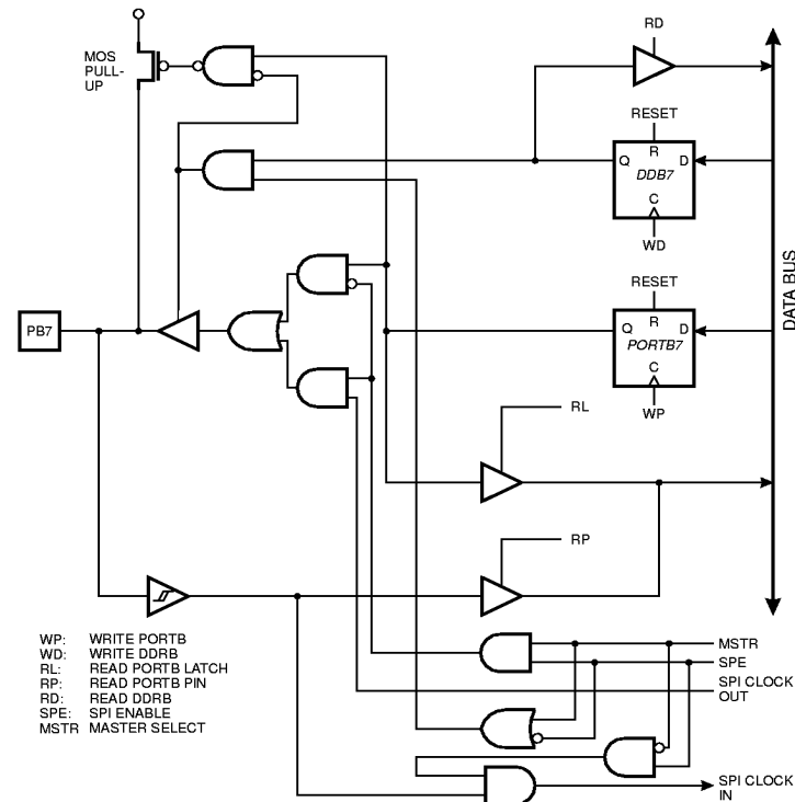
Figure 51. Port B Schematic Diagram (Pin PB7)
