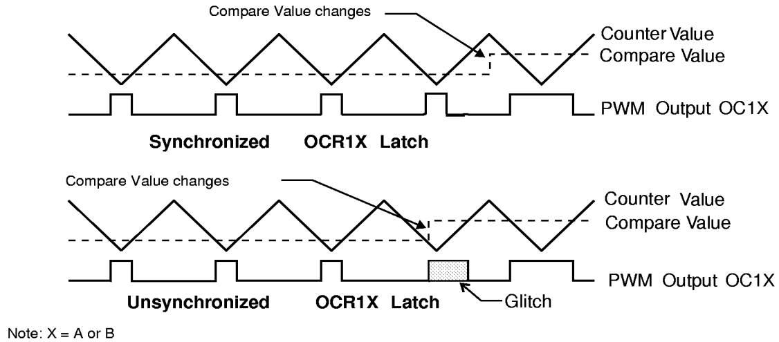
Figure 32. Effects on Unsynchronized OCR1 Latching
