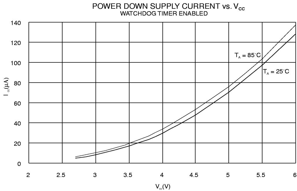
Figure 74. Power Down Supply Current vs. V_{CC}
