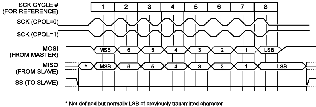
Figure 37. SPI Transfer Format with CPHA = 1 and DORD = 0
