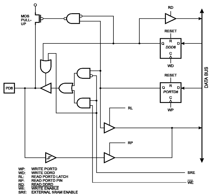
Figure 58. Port D Schematic Diagram (Pin PD6)
