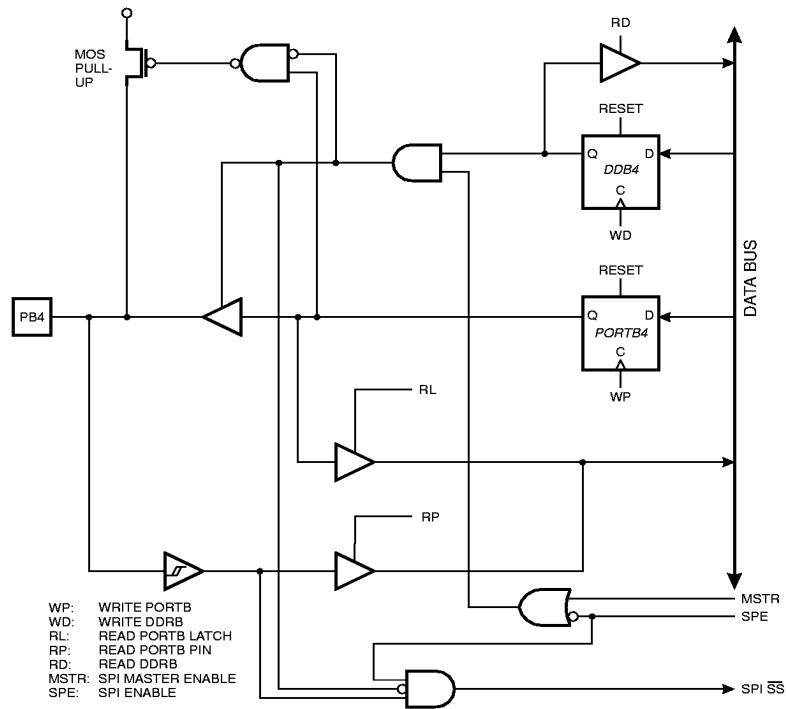
Figure 48. Port B Schematic Diagram (Pin PB4)
