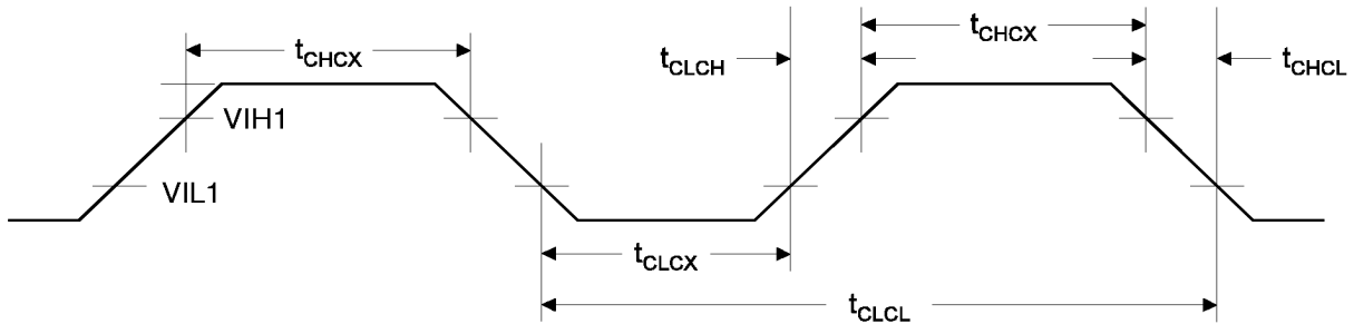
Figure 67. External Clock
