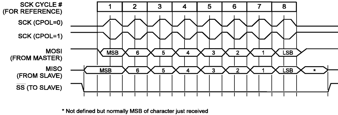
Figure 36. SPI Transfer Format with CPHA = 0 and DORD = 0
