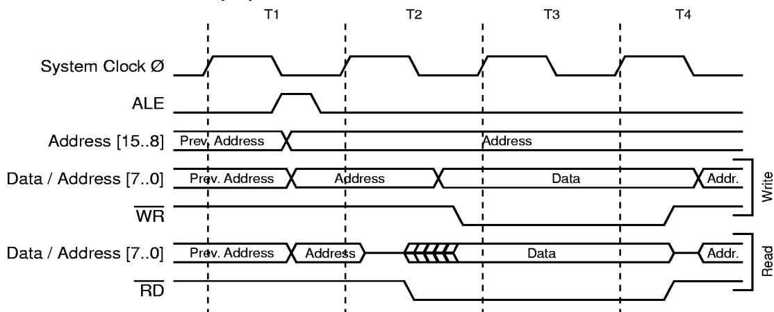
Figure 44. External Data SRAM Memory Cycles with Wait State
