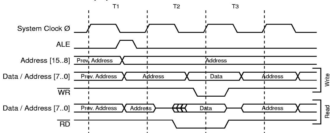
Figure 43. External Data SRAM Memory Cycles without Wait State
