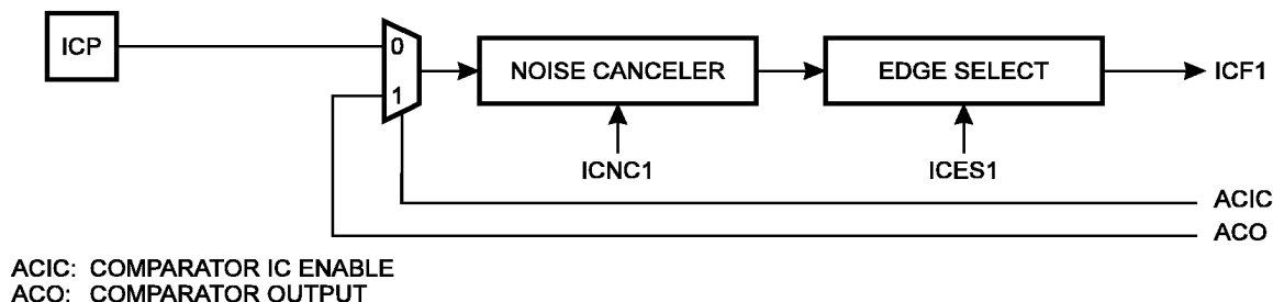
Figure 31. ICP Pin Schematic Diagram
