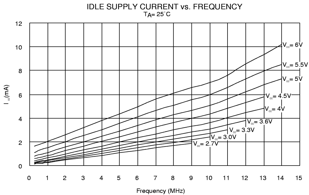
Figure 71. Idle Supply Current vs. Frequency
