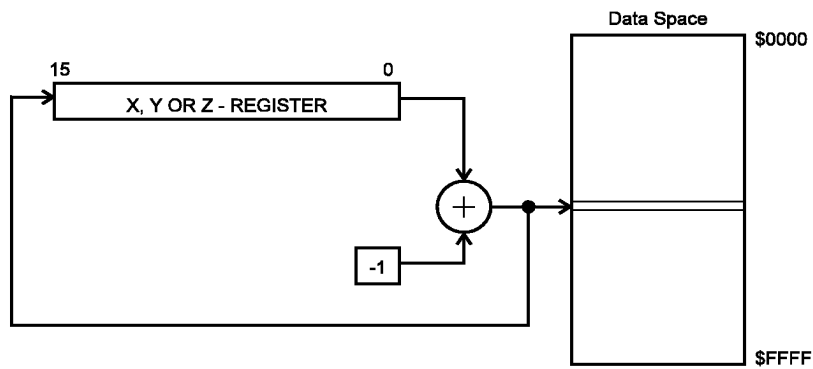
Figure 15. Data Indirect Addressing with Pre-decrement
