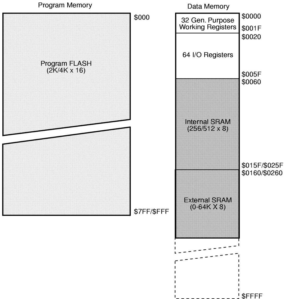
Figure 5. Memory Maps
