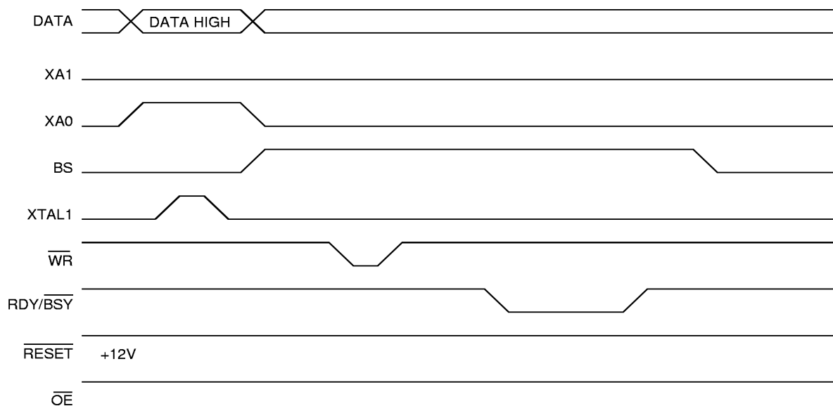
Figure 62. Programming the Flash Waveforms (continued)
