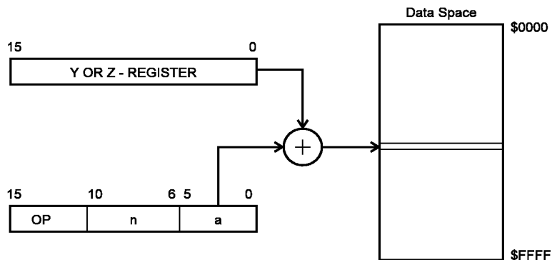
Figure 13. Data Indirect with Displacement
