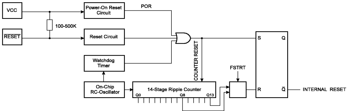
Figure 23. Reset Logic
