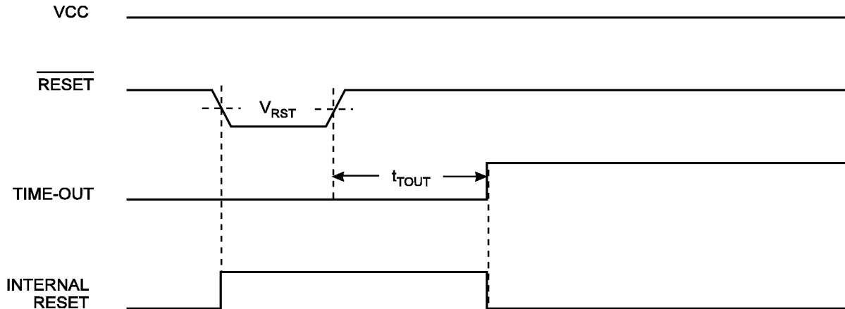
Figure 26. External Reset During Operation
