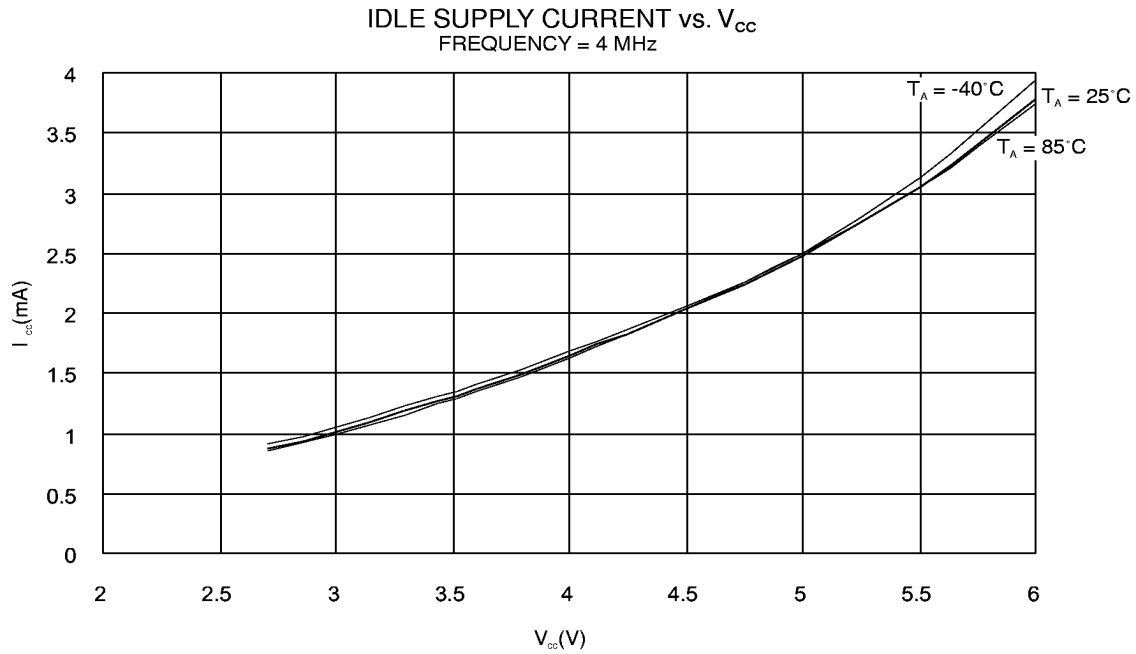
Figure 72. Idle Supply current vs. V_{CC}
