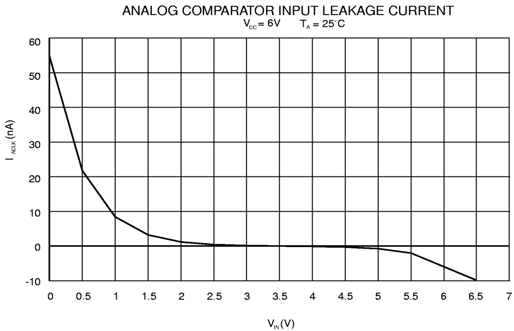
Figure 78. Analog Comparator Input Leakage Current
