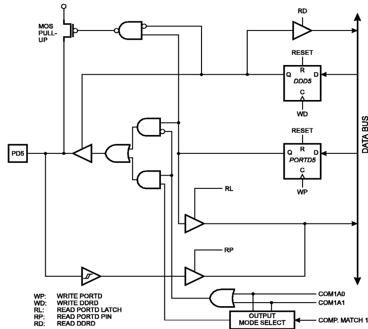
Figure 57. Port D Schematic Diagram (Pin PD5)
