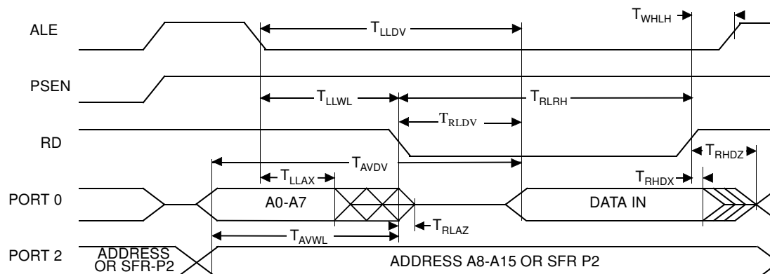
Figure 11-8. External Data Memory Read Cycle
