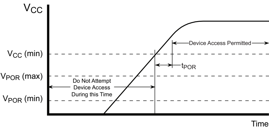
Figure 7-2. Power-Up Timing
