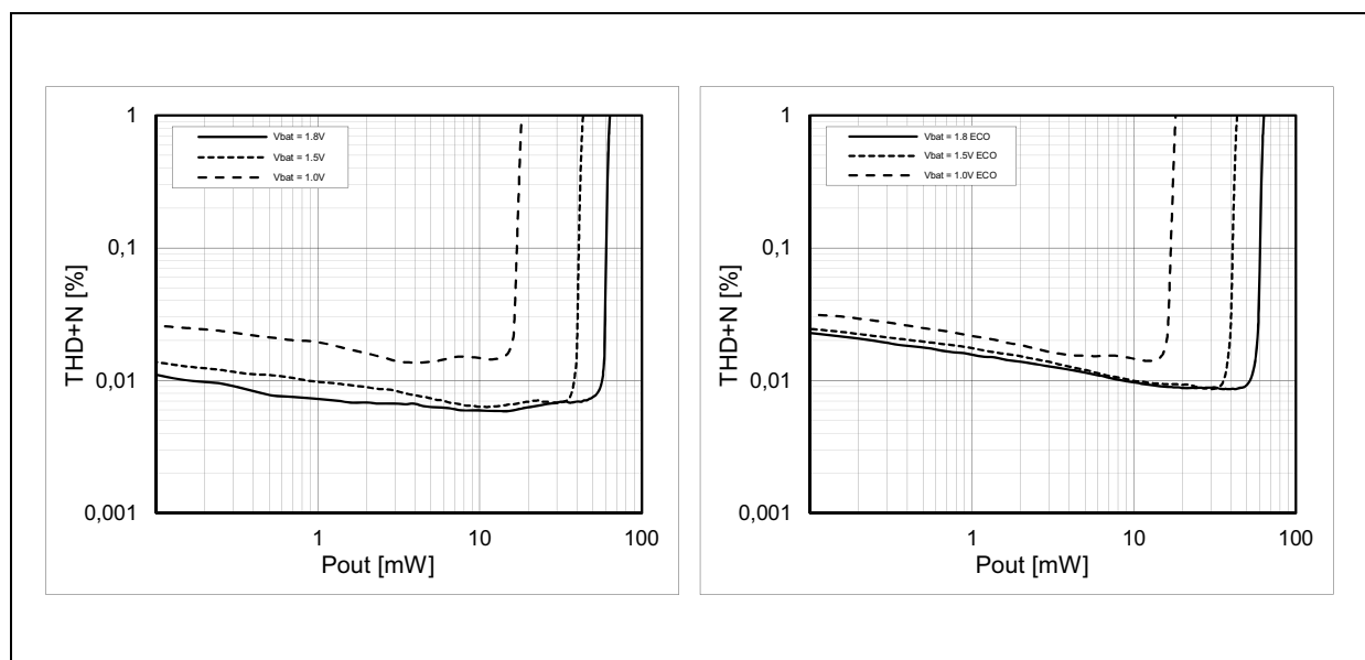
Figure 34: Headphone THD+N vs. Output Power 16 \Omega Stereo
