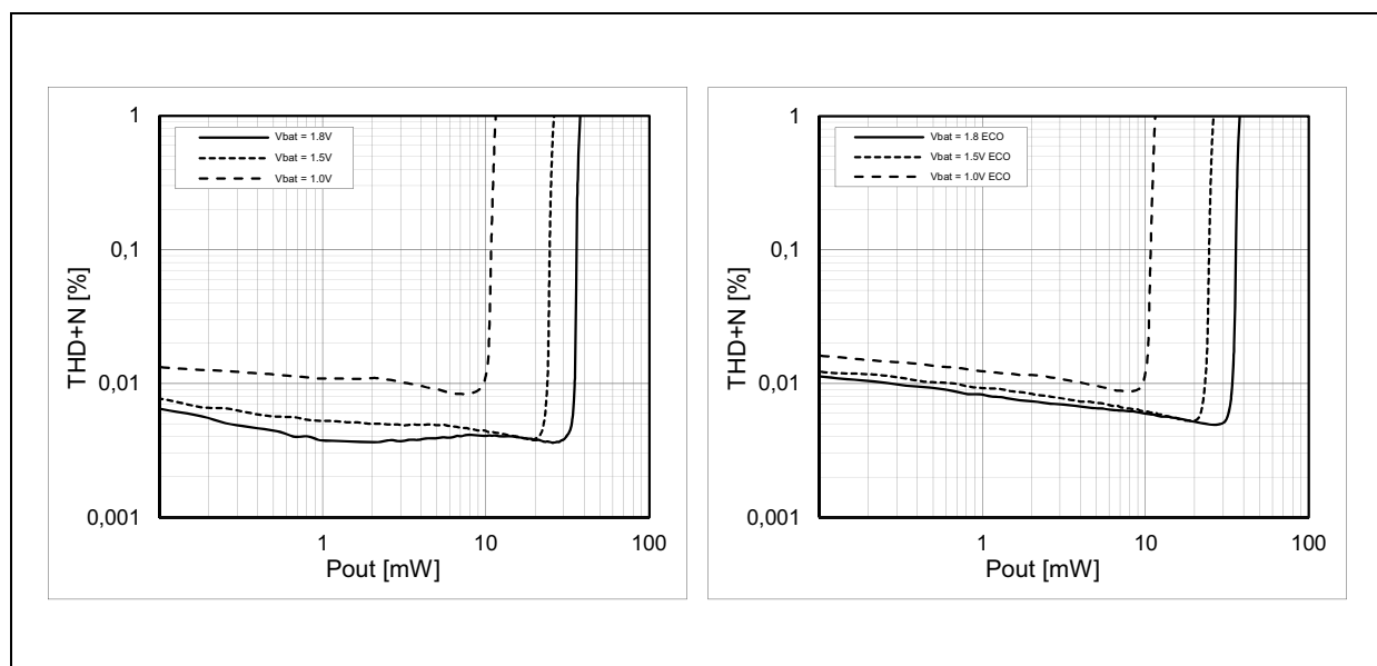
Figure 33: Headphone THD+N vs. Output Power 32 \Omega Stereo
