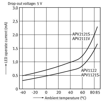
3. LED operate current vs. ambient temperature characteristics
