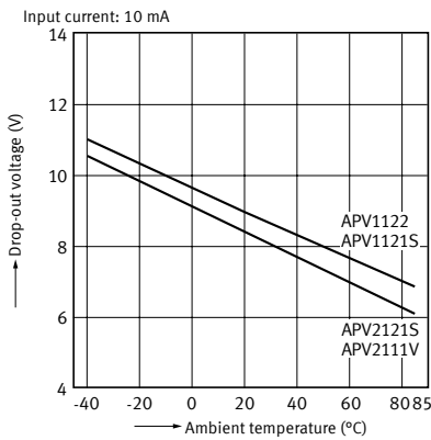
1. Drop-out voltage vs. ambient temperature characteristics
