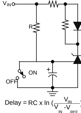
Fig. 5 Delay Timer
