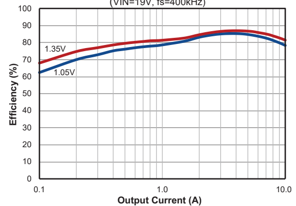
Efficiency vs. Load Current ( V_{IN}=19\text{V} , f_s=400\text{kHz} )
