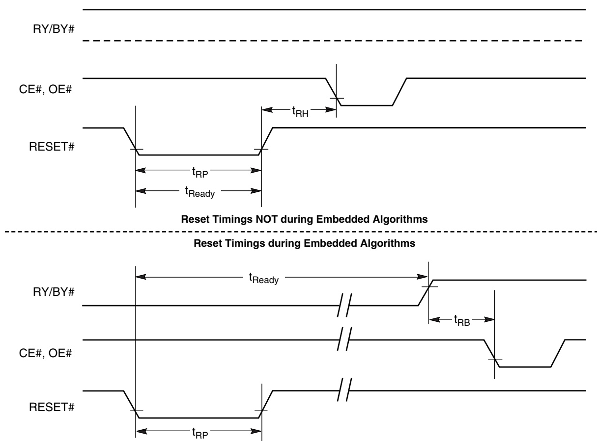
Figure 10. RESET# Timings
