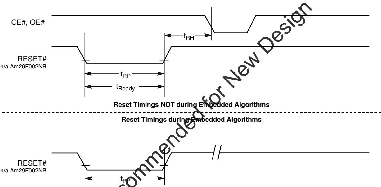
Figure 10. RESET# Timings
