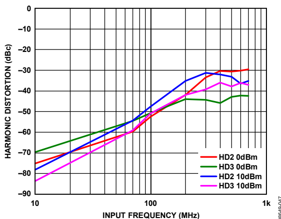
Figure 45. ADV3220 Harmonic Distortion, R_L = 100 \Omega , C_L = 4 \text{ pF}
