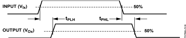
Figure 18. Propagation Delay Parameters
