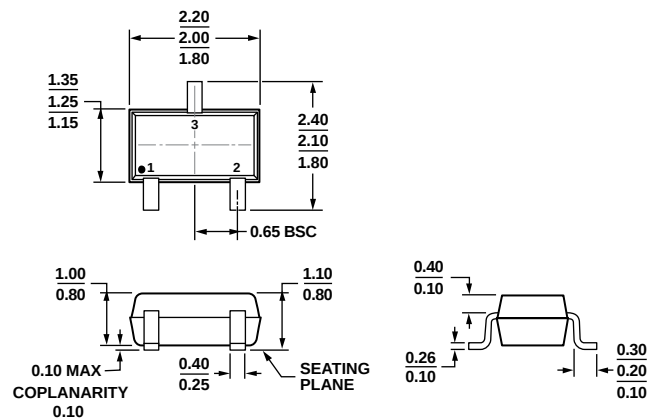
Figure 24. 3-Lead Thin Shrink Small Outline Transistor Package [KS-SC-70] (KS-3)
