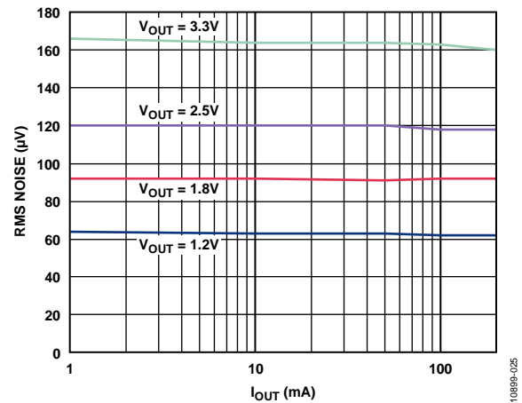
Figure 27. Channel 5 (LDO Regulator) Output Noise vs. Output Load, V_{IN} = 5\text{ V} , C_{OUT} = 1\text{ }\mu\text{F}
