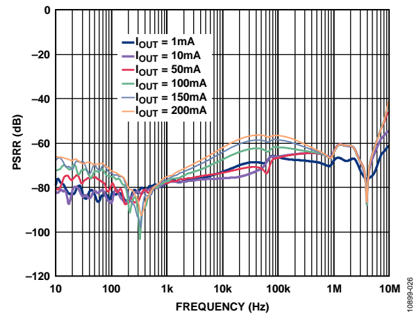
Figure 28. Channel 5 (LDO Regulator) PSRR over Output Load, V_{IN} = 5\text{ V} , V_{OUT} = 3.3\text{ V} , C_{OUT} = 1\text{ }\mu\text{F}
