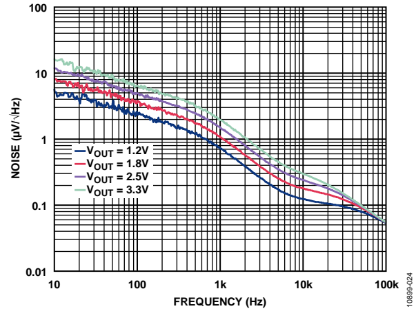
Figure 26. Channel 5 (LDO Regulator) Output Noise Spectrum, V_{IN} = 5\text{ V} , C_{OUT} = 1\text{ }\mu\text{F} , I_{OUT} = 10\text{ mA}
