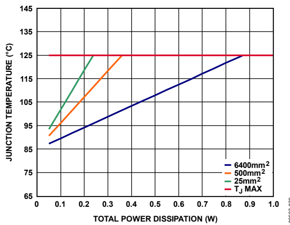
Figure 75. SOIC, T_A = 85^\circ\text{C}
