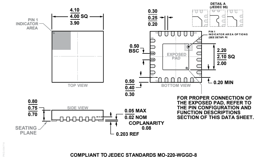
COMPLIANT TO JEDEC STANDARDS MO-220-WGGD-8 Figure 54. 24-Lead Lead Frame Chip Scale Package [LFCSP] 4 mm × 4 mm Body and 0.75 mm Package Height (CP-24-10) Dimensions shown in millimeters
