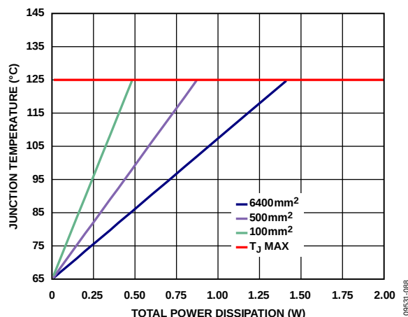
Figure 88. Junction Temperature vs. Power Dissipation, T_A = 65^\circ\text{C}
