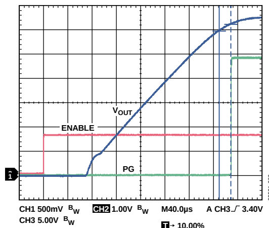
Figure 80. Typical PG Timing at Startup
