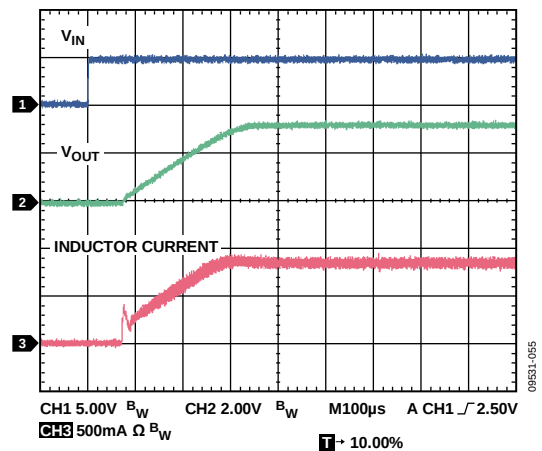
Figure 55. Startup, V_{OUT} = 3.3 V, 800 mA
