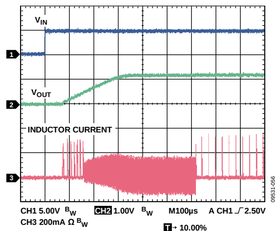
Figure 56. Startup, V_{OUT} = 1.2 V, 10 mA, V_{IN} = 5 V
