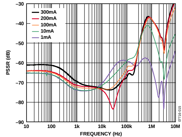
Figure 15. Power Supply Rejection Ratio vs. Frequency, V_{OUT} = 0.8 V
