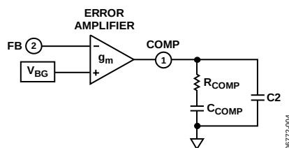
Figure 35. Compensation Components
