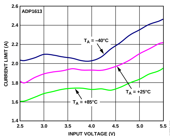
Figure 15. ADP1613 Switch Current Limit vs. Input Voltage, V_{OUT} = 15\text{ V}
