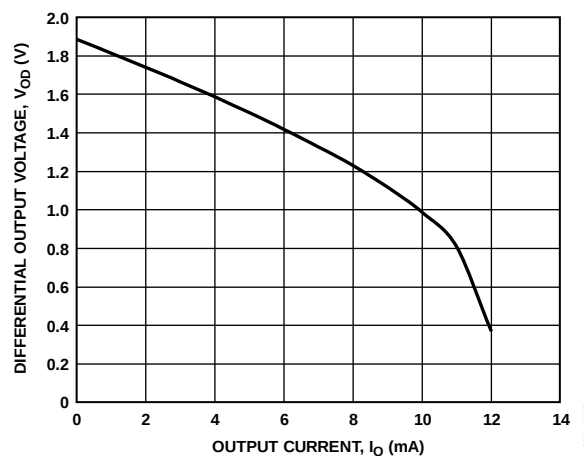
Figure 9. Driver Differential Output Voltage vs. Output Current ( V_{CC} = 3.3 V, T_A = 25^\circ\text{C} )
