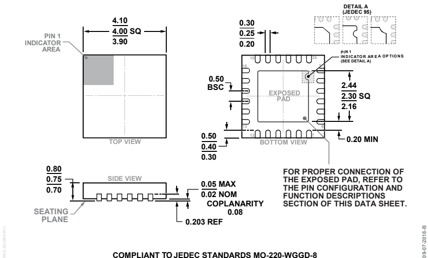
COMPLIANT TO JEDEC STANDARDS MO-220-WGGD-8 Figure 34. 24-Lead Lead Frame Chip Scale Package [LFCSP] 4 mm × 4 mm Body and 0.75 mm Package Height (CP-24-14) Dimensions shown in millimeters
