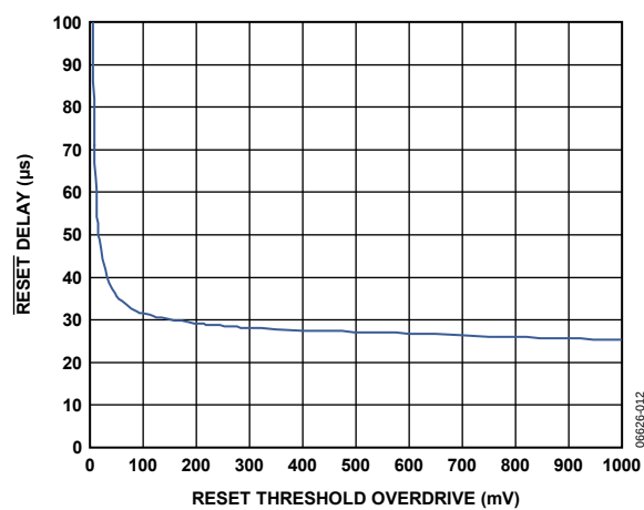
Figure 8. \overline{RESET} Delay vs. Reset Threshold Overdrive ( I_{INx} Decreasing)
