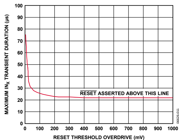
Figure 7. Maximum I_{INx} Transient Duration vs. Reset Threshold Overdrive
