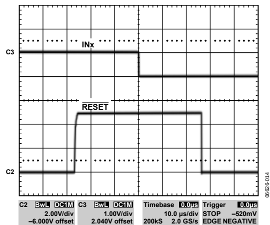
Figure 10. RESET Pull-Up and Pull-Down Response (10 \mu s/div)
