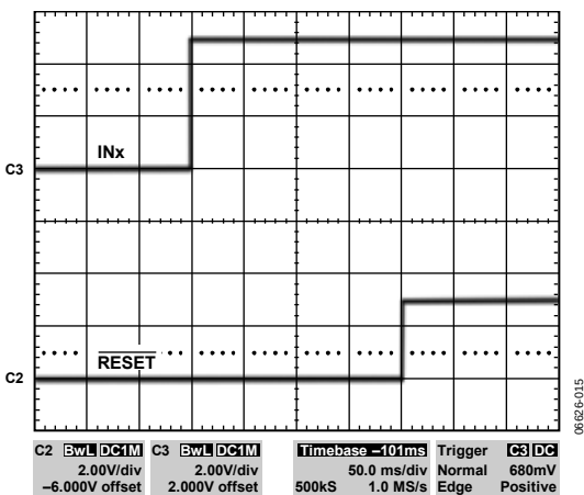
Figure 11. RESET Timeout Delay (50 ms/div)
