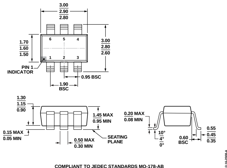
Figure 16. 6-Lead Small Outline Transistor Package [SOT-23] (RJ-6)
