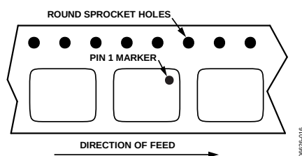
Figure 17. ADM6710 Reel Orientation
