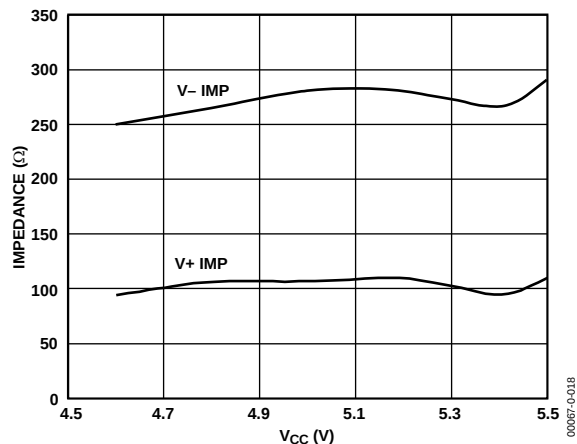
Figure 16. Charge Pump Impedance vs. V_{CC}
