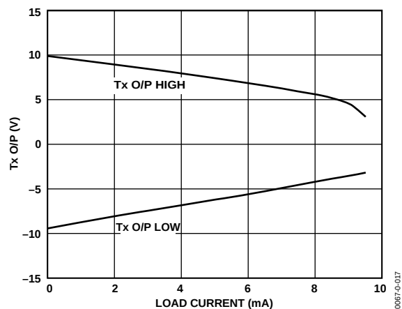
Figure 15. Transmitter Output Voltage vs. Load Current
