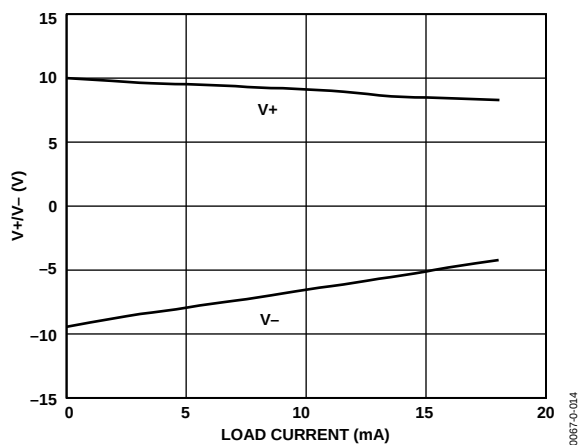
Figure 12. Charge Pump V_+ , V_- vs. Load Current
