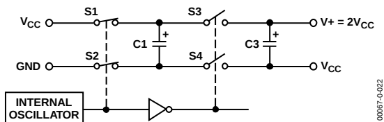
Figure 20. Charge Pump Voltage Doubler
