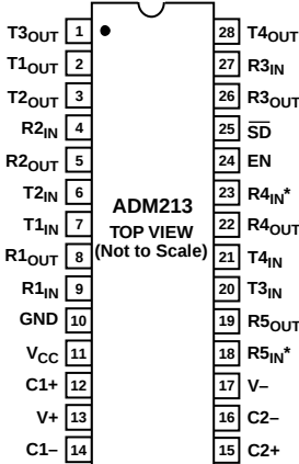
Figure 10. ADM213 SOIC/SSOP Pin Configuration
