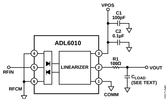
Figure 40. Basic Connections
