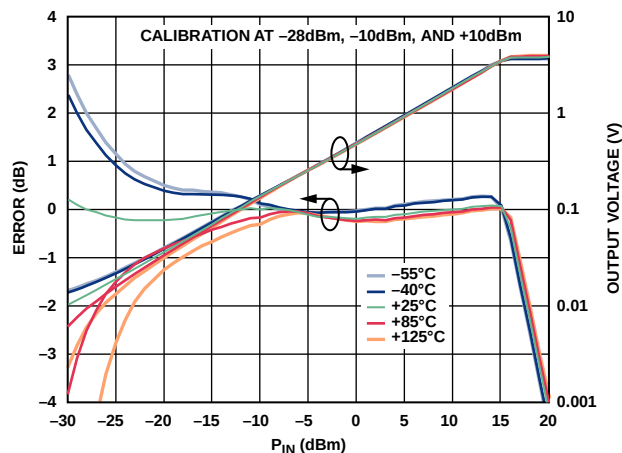
Figure 44. 10 GHz Conformance Error and Output Voltage vs. RF Input Power ( P_{IN} ) for Second Device at +25^{\circ}\text{C} , -40^{\circ}\text{C} , -55^{\circ}\text{C} , +85^{\circ}\text{C} , and +125^{\circ}\text{C}
