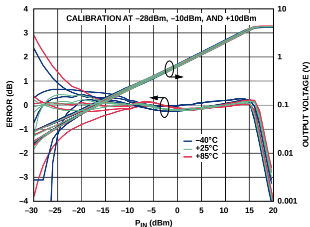
Figure 45. 10 GHz Conformance Error and Output Voltage vs. RF Input Power ( P_{IN} ) at +25^{\circ}\text{C} , +85^{\circ}\text{C} , and -40^{\circ}\text{C} for Multiple Devices
