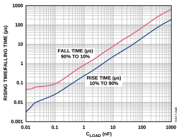
Figure 46. Rising Time/Falling Time vs. C_{LOAD} for a 1 GHz Modulated Pulsed Waveform with P_{IN} = 0 dBm
