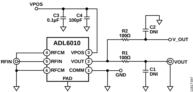
Figure 47. ADL6010 Evaluation Board Schematic
