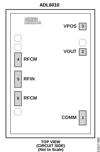
Figure 3. 6-Pad Bare Die Pin Configuration
