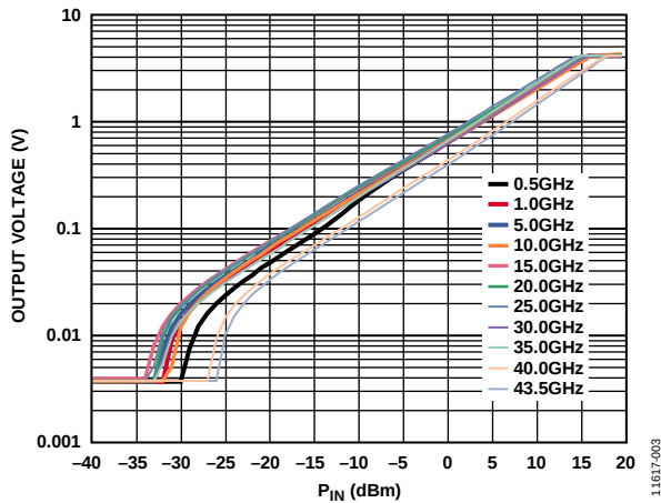
Figure 4. Typical Output Voltage ( V_{OUT} ) vs. RF Input Power ( P_{IN} ) at Various Frequencies (0.5 GHz to 43.5 GHz) at 25^\circ\text{C}
