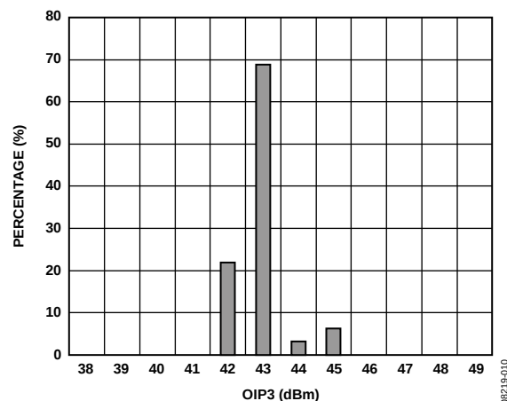
Figure 12. OIP3 Distribution at 900 MHz, P_{OUT} = 0 dBm
