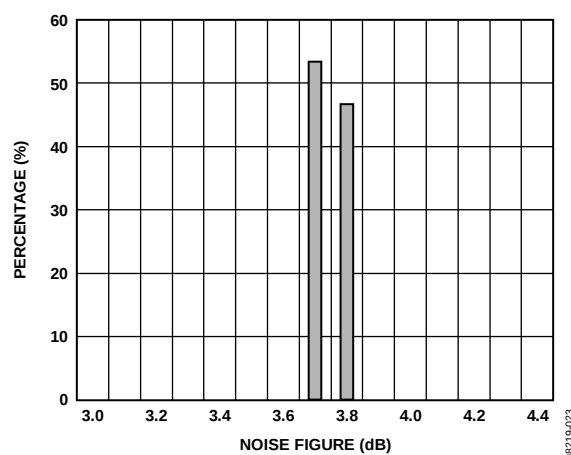
Figure 13. Noise Figure Distribution at 900 MHz
