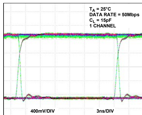
Figure 26. Eye Diagram at A Output (3.3 V to 1.8 V Level Translation, 50 Mbps)
