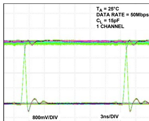
Figure 28. Eye Diagram at A Output (5 V to 3.3 V Level Translation, 50 Mbps)
