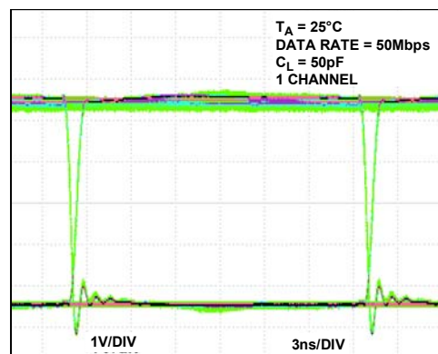
Figure 27. Eye Diagram at Y Output (3.3 V to 5 V Level Translation, 50 Mbps)
