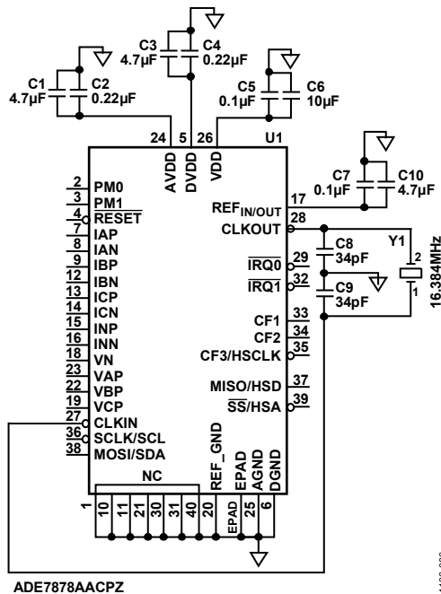
Figure 91. ADE7878A Crystal and Capacitor Connections
