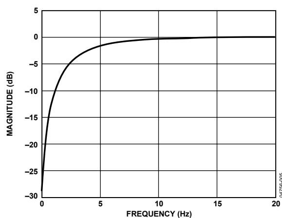
Figure 5. ADC High-Pass Filter Response, f_s = 96 kHz
