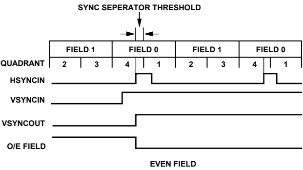
Figure 12. Even Field
