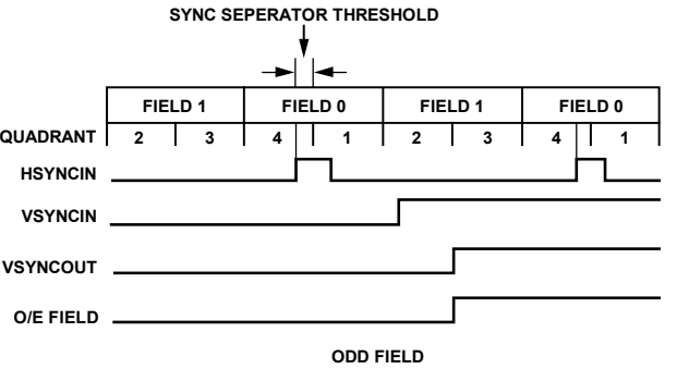
Figure 13. Odd Field
