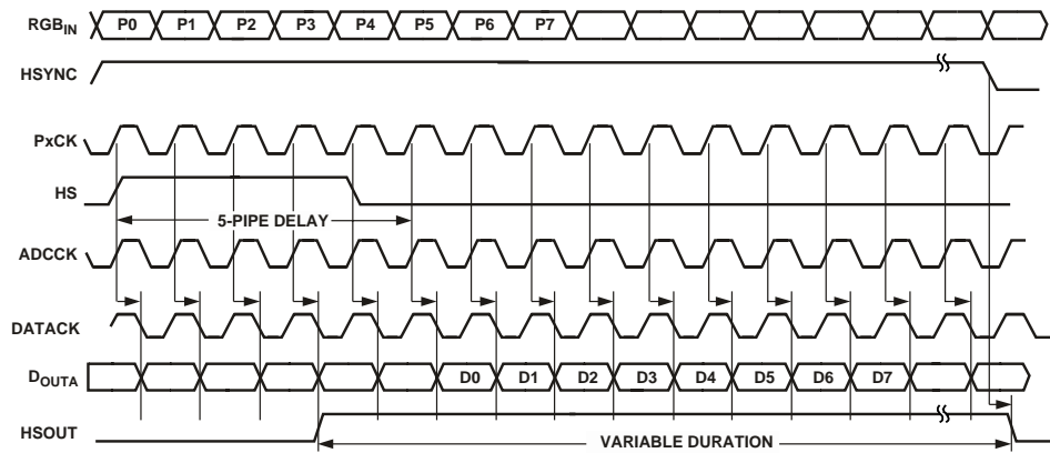
Figure 10. 4:4:4 Mode (For RGB and YUV)
