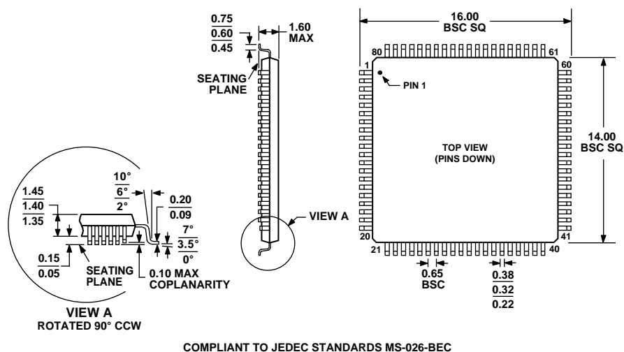
Figure 16. 80-Lead Low Profile Quad Flat Package (LQFP)
