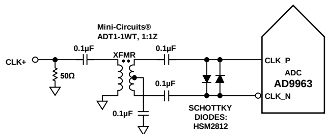
Figure 69. Transformer Coupled Clock
