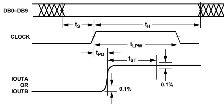
Figure 2. Timing Diagram
