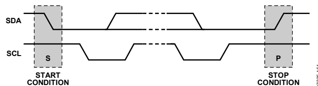
Figure 58. Start and Stop Conditions
