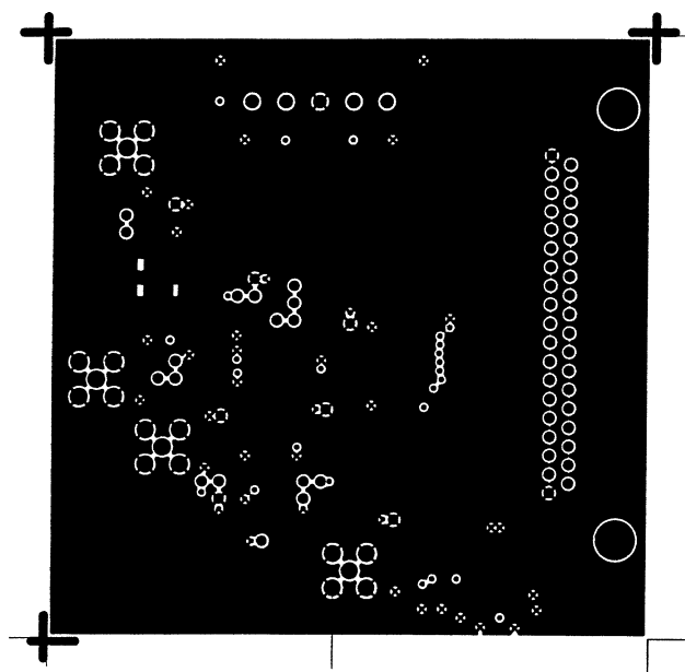
Figure 11. Printed Circuit Board Ground Layer
