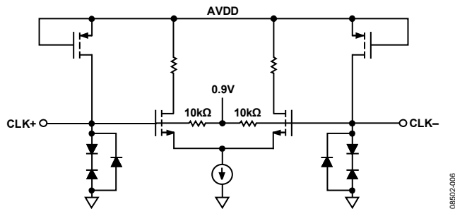
Figure 54. Equivalent Clock Input Circuit
