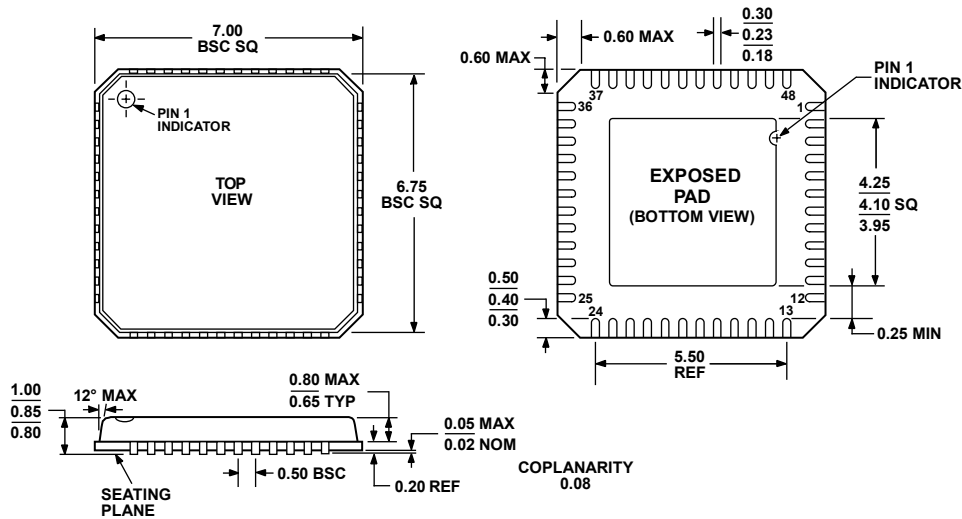
COMPLIANT TO JEDEC STANDARDS MO-220-VKDD-2 Figure 64. 48-Lead Lead Frame Chip Scale Package [LFCSP_VQ] 7 mm × 7 mm Body, Very Thin Quad (CP-48-3) Dimensions shown in millimeters
