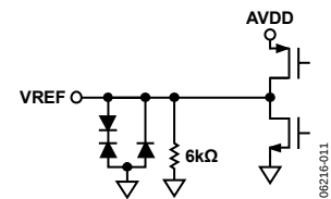
Figure 11. Equivalent VREF Circuit
