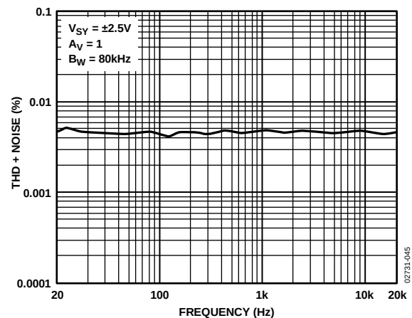
Figure 48. THD + Noise vs. Frequency
