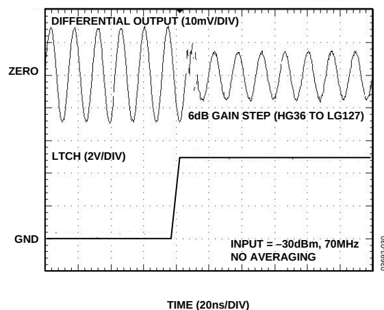
Figure 32. Gain Step Time Domain Response
