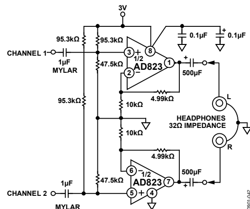
Figure 42. 3 V Single-Supply Stereo Headphone Driver
