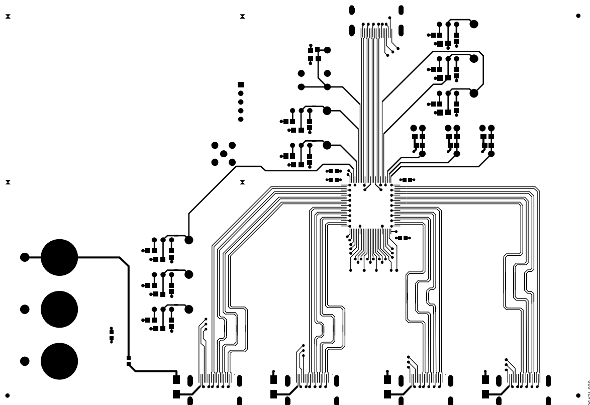
Figure 31. Layout of the TMDS Traces on the AD8197 Evaluation Board (Only Top Signal Routing Layer is Shown)
